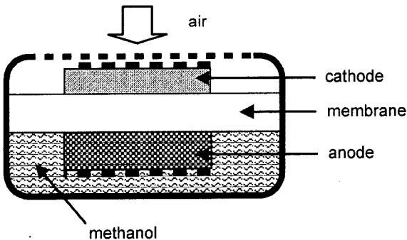
Fig. 1. Schematic diagram of an passive & air-breathing cell of DMFC.
