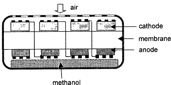
Fig. 2. Schematic diagram of an monopolar stack of DMFC.
