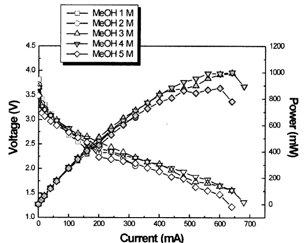
Fig. 6. Performance of the monopolar stack with 6 cells having 6 cm 2 per cell. MeOH/air, R.T.
