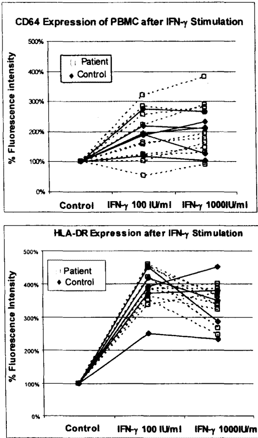
Fig. 2. The fluorescence intensity pattern of PBMC with or without IFN- \gamma stimulation in all subjects. The baseline mean fluorescence intensity was set at 100% and the increased fluorescent intensity was expressed as a % of the baseline intensity.
