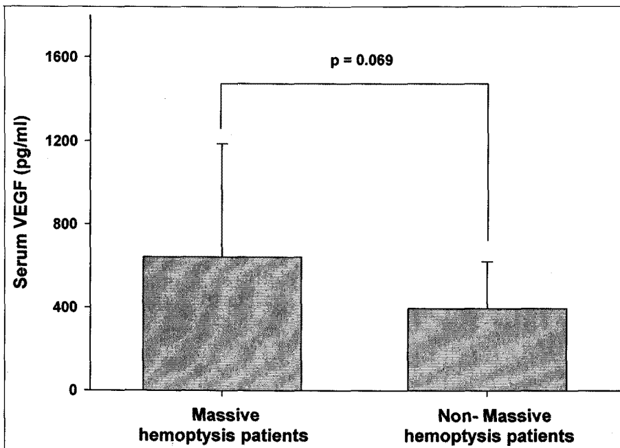
Fig. 2. Comparison of serum VEGF concentration according to the amount of hemoptysis.
