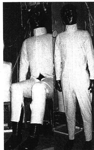
Fig. 2. The clothed thermal manikin in standing/seated pose
