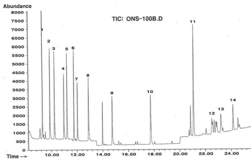
Fig. 2. Total ion chromatogram of organonitrogen pesticides obtained from standard solutions.
