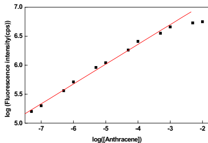
Fig. 5. Calibration curves for anthracene in synthetic mixture solution: [anthracene] = 1.0 \times 10^{-3} M ~ 1.0 \times 10^{-8} M, [fluorene] = 1.0 \times 10^{-4} M.
