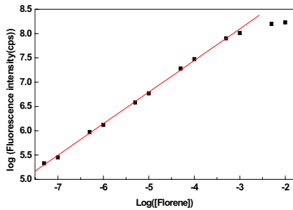
Fig. 4. Calibration curves for fluorene in synthetic mixture solution: [fluorene] = 1.0 \times 10^{-3} M ~ 1.0 \times 10^{-8} M, [anthracene] = 1.0 \times 10^{-4} M.
