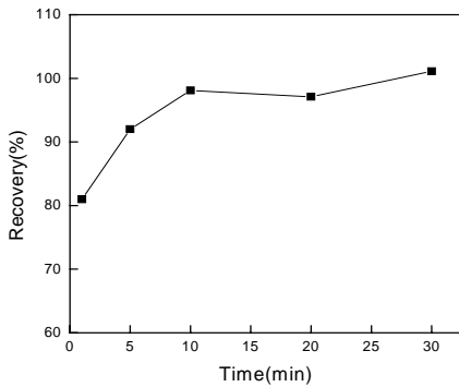
Fig. 8. Effect of extraction time on extraction of Ce: pH, 4.3.
