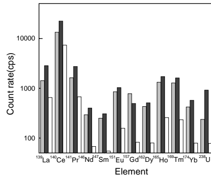
Fig. 1. Response of ion counts for blank solutions: □; EtOH, ■; EtOH-IMBK, ▒; MIBK-EtOH-0.03 M HEH.
