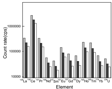
Fig. 2. Response of ion counts for 20 ng/mL rare earth elements in each solvent: □; EtOH, ■; EtOH-IMBK, ▒; MIBK-EtOH-0.03 M HEH.
