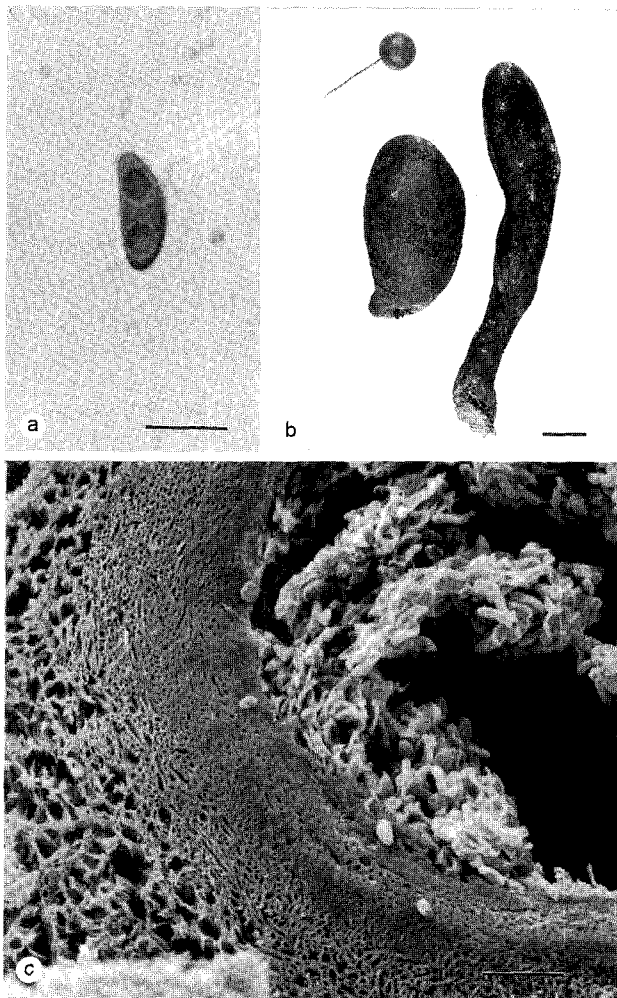
Fig. 1. Light micrographs (a, b) and scanning electron micrographs (c) of Xylaria allantoidea . a. Ascospores with oil guttule (bar: 10 \mu\text{m} ). b. Stromata cylindrical allantoid and clavate (bar: 10 \mu\text{m} ). c. Cross section of ascoma, inner layer of thick cell walls and an outer layer more mycelial in appearance. Released ascospores in the centrum (bar: 10 \mu\text{m} ).
