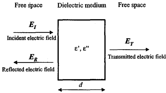
Fig. 1 A general schematic diagram of the electric field and dielectric material
