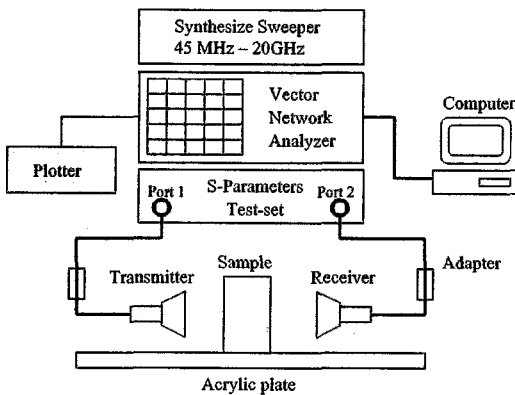
Fig. 2 Free-space transmission measurement system
