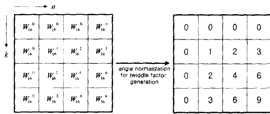
Fig 5. Twiddle factor generation method for the 16-point DFT.
