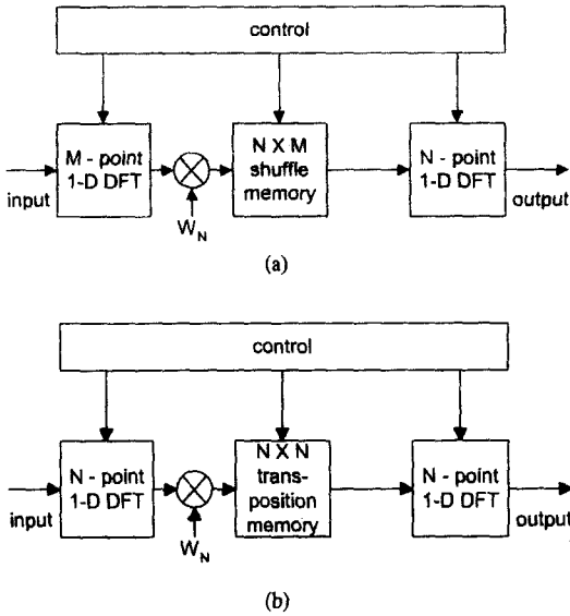
Fig 2. Basic building blocks of the proposed system based on the Cooley-Tukey algorithm (a) using the shuffle memory, (b) using the transposition memory.
