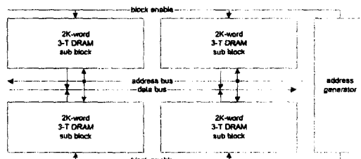
Fig. 8 Structure of the 8K-word shuffle memory.
