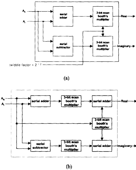
Fig 4. (a) Complex multiplier with two real multiplications. (b) Complex multiplier with three real multiplications.
