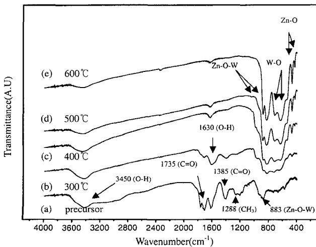
Fig. 3. FT-IR spectra of the (a) precursor and powders heat-treated at (b) 300, (c) 400, (d) 500 and (e) 600°C for 3 h.
