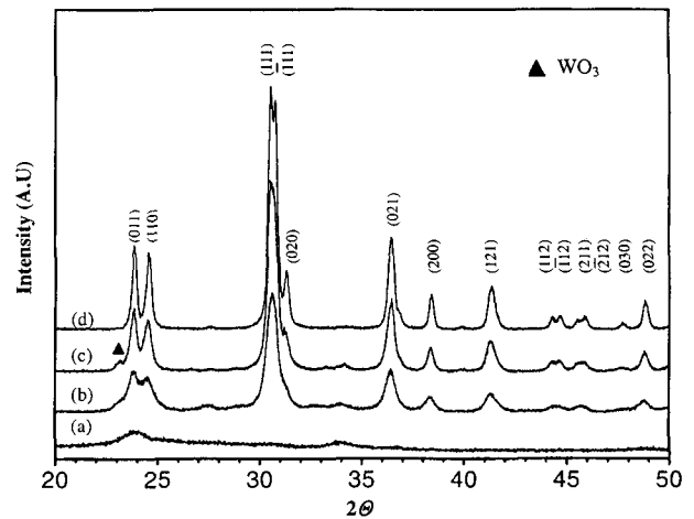
Fig. 1. XRD patterns of the powders heat-treated at (a) 300^\circ C , (b) 400^\circ C , (c) 500^\circ C and (d) 600^\circ C for 3 h.
