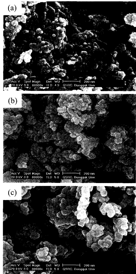
Fig. 4. Scanning electron micrographs of ZnWO 4 nanopowders calcined at (a) 400, (b) 500 and (c) 600°C for 3 h.
