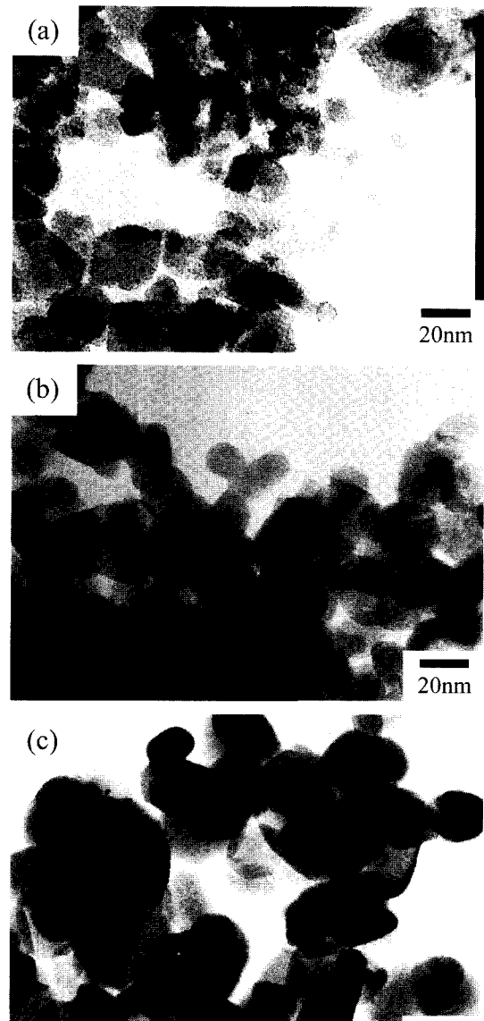
Fig. 5. Transmission electron micrographs of \text{ZnWO}_4 nanocrystalline powders heat-treated at (a) 400, (b) 500 and (c) 600°C for 3 h.
