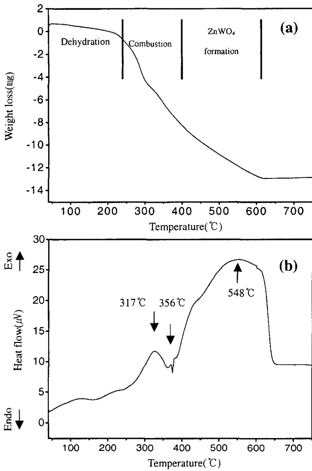
Fig. 2. (a) TGA curves and (b) DTA curves of the precursor in flowing air.
