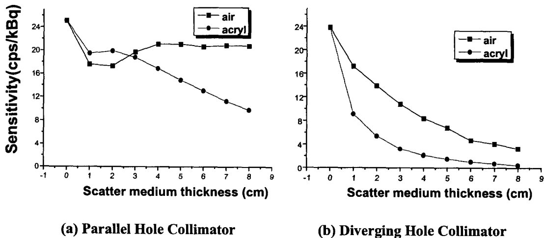
Fig. 2. Sensitivity vs. medium thickness for different types of collimator and media. The result of simulation.
