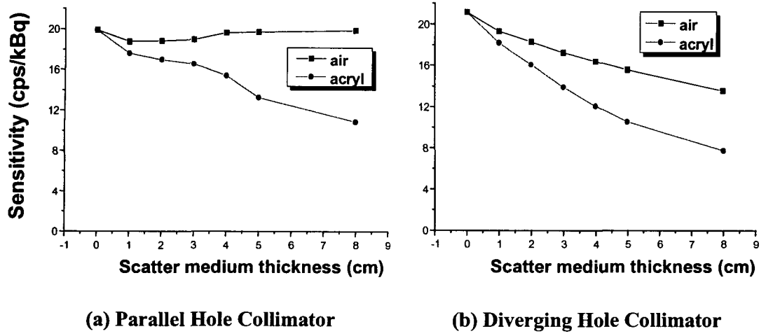
Fig. 3. Sensitivity vs. medium thickness for different types of collimator and media. The result of experiment.
