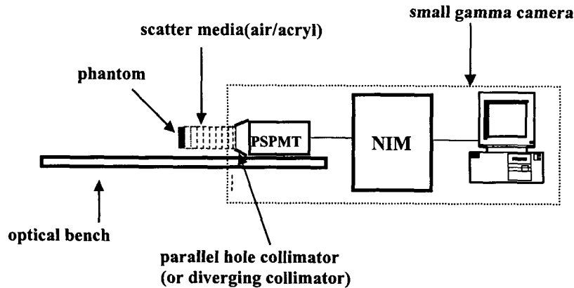
Fig. 1. Experiment setup for Monte Carlo simulation and measurement.
