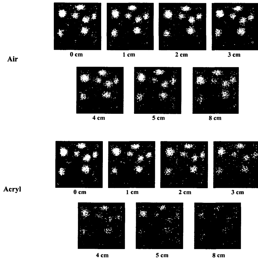
Fig. 4. Images for different media thickness. Two kinds of media (air, acryl) and parallel hole collimator was used.
