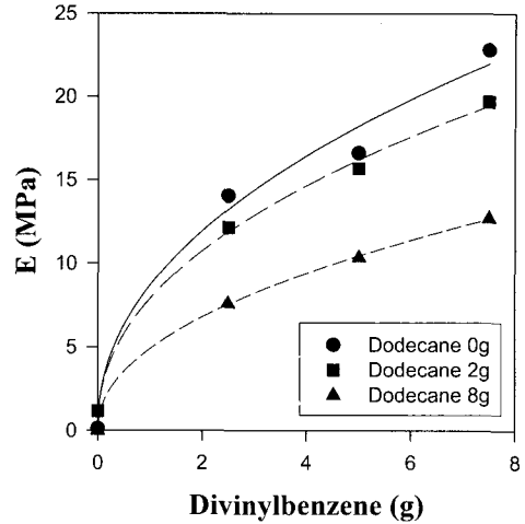
Figure 9. Effect of divinylbenzene content on compression modulus (D-series).
