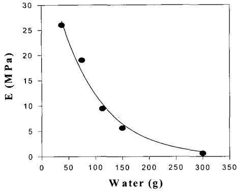
Figure 3. Effect of water content on compression modulus (W-series).
