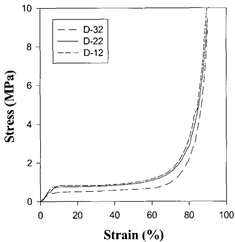
Figure 6. Compression stress-strain curves of microcellular foams showing the effect of dodecane content : D-12, D-22, D-32.
