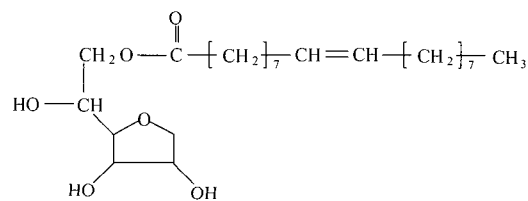
Figure 1. Chemical structure of sorbitan monooleate.
