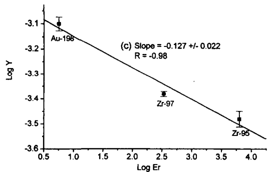
Fig. 2. The Result of \alpha -determination by "Cd-ratio triple-monitor" Method. ( Y = (E\gamma_i)^{-\alpha} / [(F_{cd,i} \cdot R_{cd,i} - 1) \cdot Q_{0,i}(\alpha) \cdot (G_{e,i}/G_{th,i})] )
