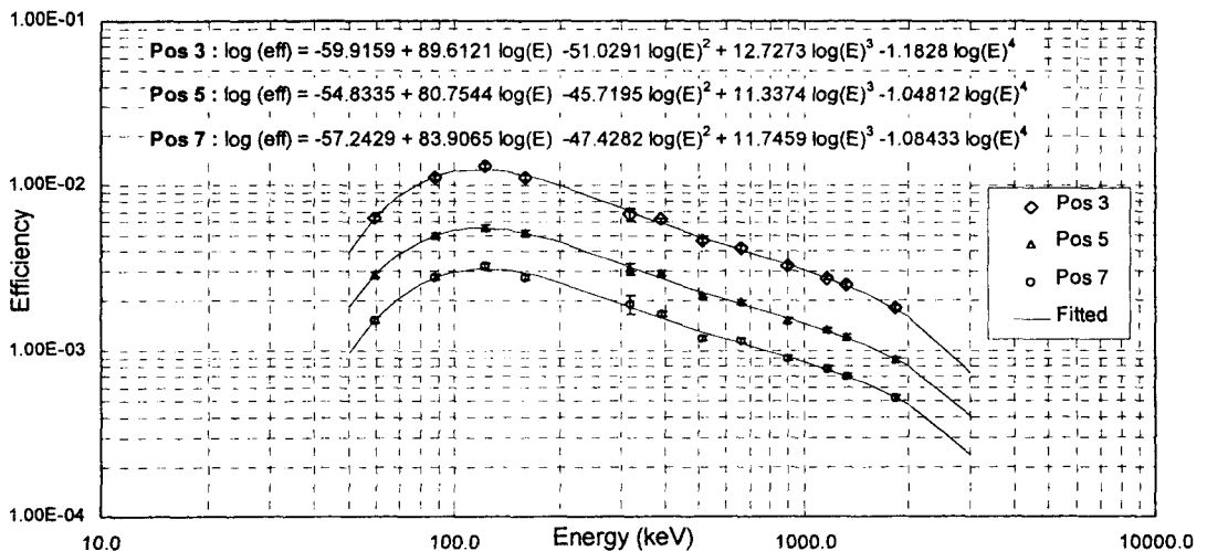
Fig. 1. Efficiency Curve of the HPGe Detector(EG & G ORTEC, GEM35185) for Three Measurement Positions
