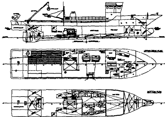
Fig. 1 General arrangement of main vessel
