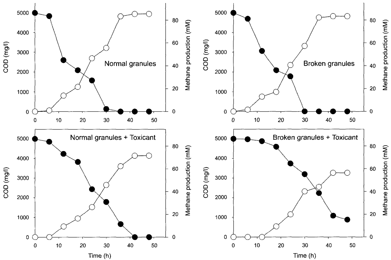
Fig. 2. Removal of COD and production of methane by intact and disintegrated granules in media containing 0 and 1 unit toxicant concentrations.
