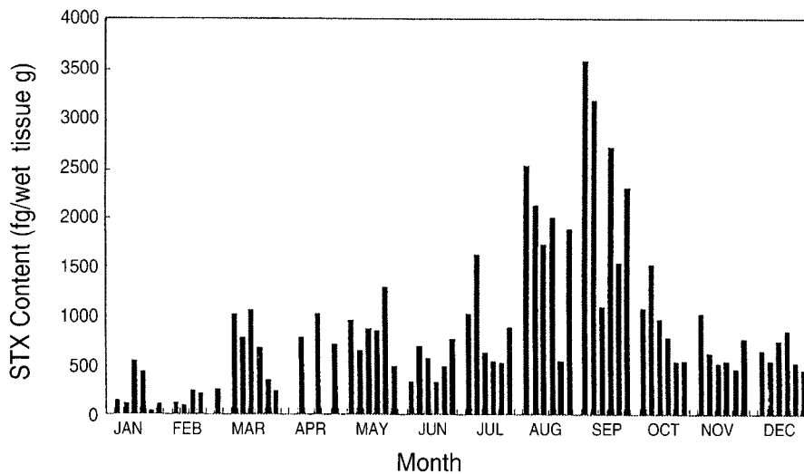
Fig. 8. Annual changes of Na + channel blocker contents in short-necked clam(Conditions are the same as in Fig. 7).
