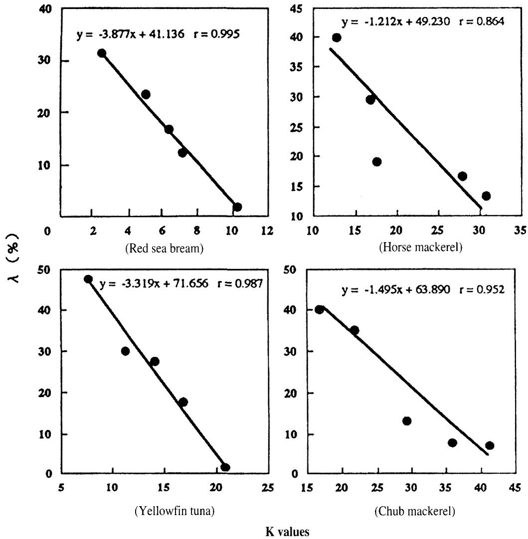
Fig. 3. Correlations between K values and \lambda values of species of fish. Conditions (heating temperature, 50 °C : heating hours, 5 min).
