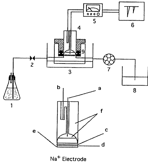
Fig. 6. Schematic diagram of the tissue biosensor flow system used for determination of GTX, STX and TTX toxicity. Ice: —, OTC-ice —. 1, 8% NaCl pH 4.8 tank; 2, injection port; 3, thermostatically controlled bath; 4, Na + electrode; 5, electrometer; 6, recorder; 7, peristaltic pump; 8, 10 N NaOH resevior. a, working electrode; b, reference electrode; c, cellulose acetate membrane; d, frog bladder membrane; e, cellulose acetate membrane; f, 1 M NH 4 Cl.
