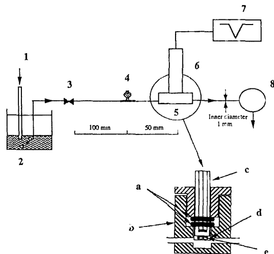
Fig. 1. Schematic diagram of TMA biosensor system(1, Air; 2, Buffer tank; 3, Injection port; 4, Gas reservoir; 5, Flow cell; 6, Oxygen electrode; 7, Recorder; 8, Peristaltic pump; a, Rubber ring; b, Flow cell; c, oxygen electrode; d, Teflon membrane and Dialysis membrane; e, Immobilized microbial membrane).
