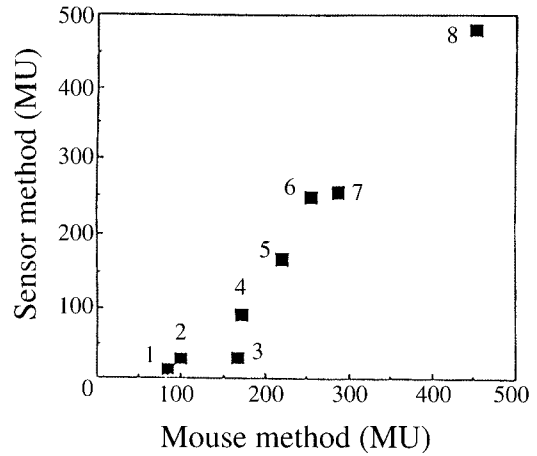
Fig. 7. Correlation between TTX activities determined by the sensor and the mouse method. Conditions: Temperature 30°C, pH 4.8, Flow rate 0.8 mL/min, Nac concn 8.0 %, Sample 50 \mu L. 1, Takifugu niphobles muscle; 2, Takifugu pardalis muscle; 3, Takifugu pardalis ovary; 4, Takifugu niphobles skin; 5, Takifugu niphobles hepatic; 6, Takifugu pardalis skin; 7, Takifugu pardales hepatic; 8, Takifugu niphobles ovary.
