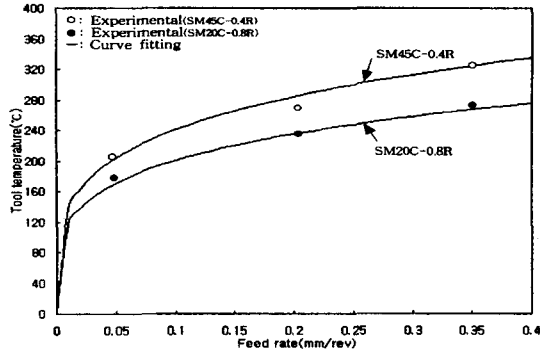
Fig. 6 Tool temperature and feed rate, depth of cut 0.3mm, cutting speed 200m/min
