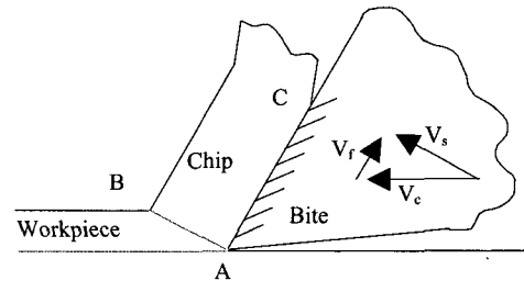
Fig. 1 Tool and chip velocity relation
