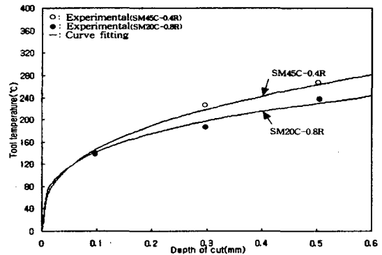
Fig. 4 Tool temperature vs. depth of cut, feed rate 0.35 mm/rev, cutting speed 80m/min
