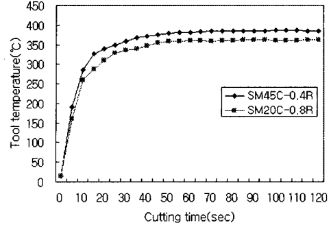
Fig. 3 Tool temperature vs. cutting time, cutting speed 200m/min, feed rate 0.35mm/rev, depth of cut 0.5mm10sec
