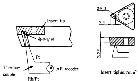
Fig. 2 Thermo-couple set-up into a bite
