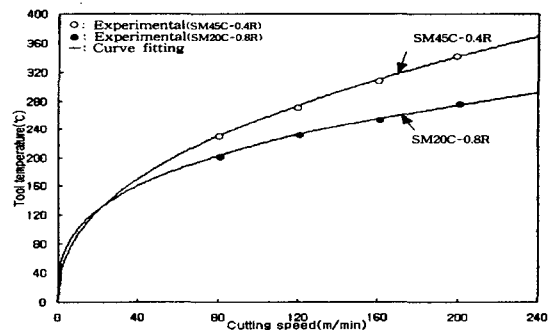
Fig. 5 Tool temperature vs. cutting speed, depth of cut 0.5mm, feed rate 0.2mm/rev
