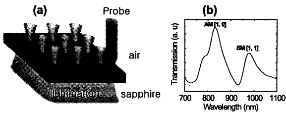
FIG. 1. (a) Schematics of our experiment (b) Transmission spectrum of a gold sample with period=760 nm, hole size=250 nm, and film thickness=200 nm.
