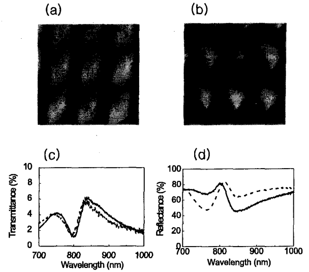
FIG. 4. Comparison of air-silver [1,0] mode and sapphire-silver [-1,1] mode. Holes with 250 nm diameter were made on 200 nm thick silver films with a period of 600 nm. Emission patterns of the air-metal [1,0] mode using \lambda = 730 nm. (b) Emission patterns of the sapphire-metal [1,1] resonance using \lambda = 830 nm. (c) Far-field transmission spectrum for the said silver sample. Dotted lines: Transmission spectrum when the incident light is from the air side. (d) Far-field reflection spectrum taken from the sapphire side in the same case as (c). Dotted lines: Reflection spectrum when the incident light is from the air side.
