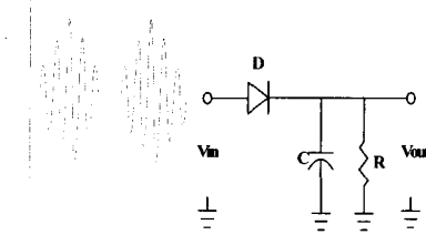
Fig. 4 Schematic of the envelope detection.
