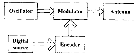
Fig. 2 Block diagram of the transmitting device.
