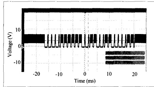
Fig. 12 Result of the envelope detection.
