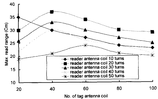
Fig. 20 Read range of developed electronic identification unit.
