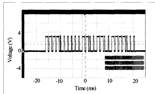
Fig. 13 Demodulated signal.
