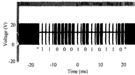
Fig. 9 Result of the modulating circuit.
