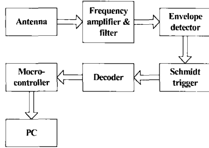
Fig. 3 Block diagram of the receiving device.
