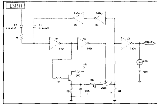
Fig. 17 Schematic of switching circuit.
