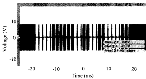
Fig. 11 High frequency amplified wave.
