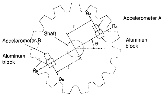
Fig. 2 Mounting position of the accelerometers
