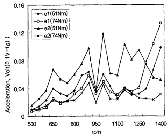
Fig. 10 Third harmonic of vibration (tooth error I and II)
