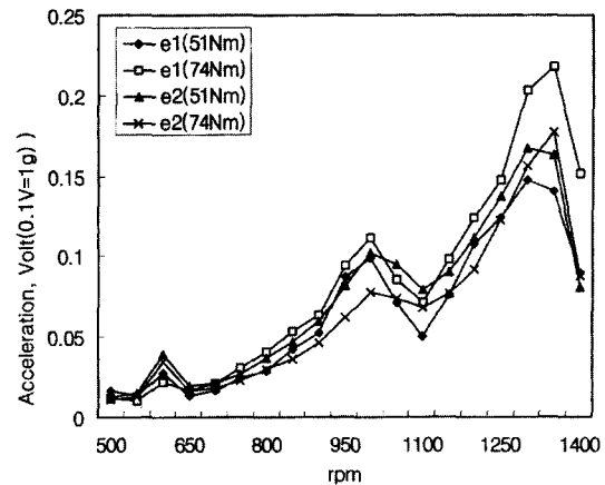
Fig. 9 Second harmonic of vibration (tooth error I and II)
