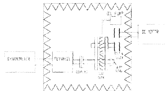
Fig. 1 Experimental apparatus layout
