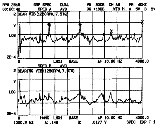
Fig. 14 Gear and bearing frequency spectrum with tooth error I (1250 rpm, 74 Nm)
