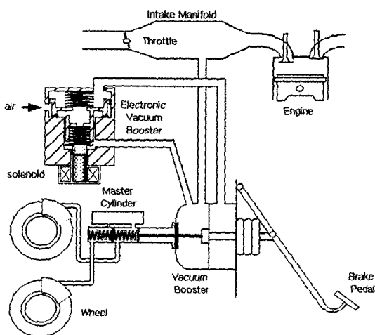
Fig. 1 Schematic diagram of an EVB controlled brake system
