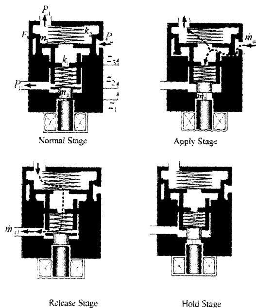
Fig. 2 Operational stages of the EVB control valve
