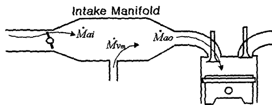
Fig. 3 Two state engine model
