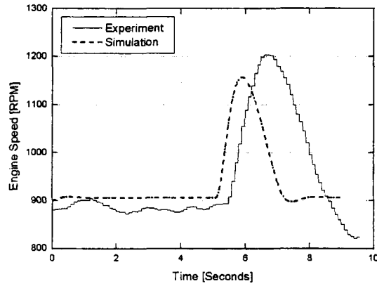
(b) Engine speed
