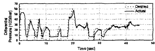
(e) Differential pressure
