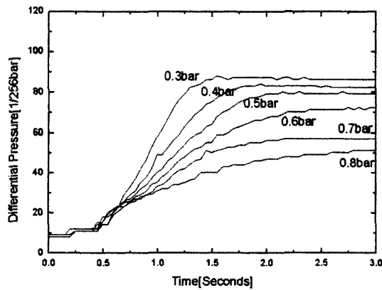
Fig. 7 Differential pressures with change of intake manifold pressure
