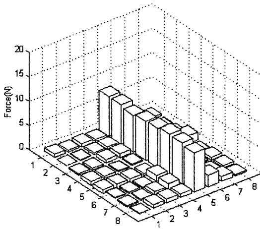
Fig. 9 Sensor response in case of bar-shape contact
