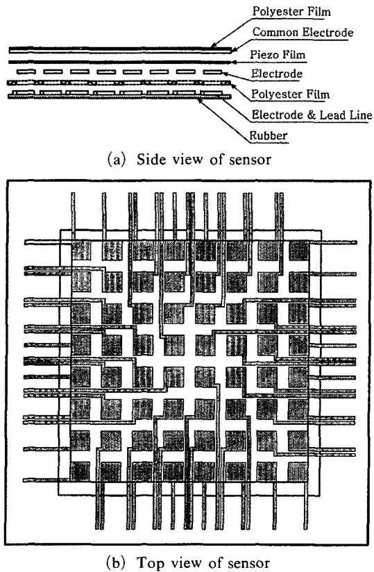
Fig. 2 Structure of tactile sensor
