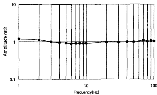
Fig. 8 Frequency response of sensor
