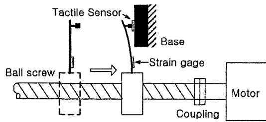
Fig. 4 Experiments for sensor calibration
