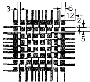
(a) Electrode and lead line
