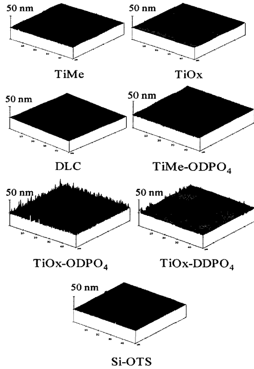
Fig. 4. 3-D surface images of the specimens measured by tapping mode AFM.
