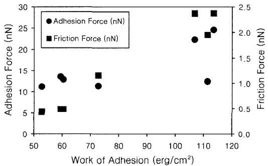
Fig. 11. Adhesion and friction force vs. the work of adhesion.
