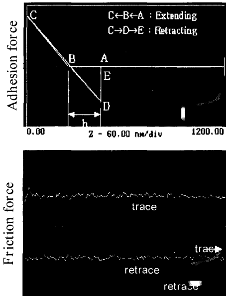
Fig. 2. Schematic illustration of the measurement of adhesion and friction force.
