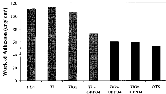
Fig. 6. Work of adhesion of the specimens.
