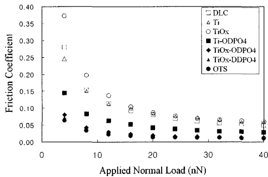
Fig. 9. Coefficient of friction of specimens with the applied normal load.
