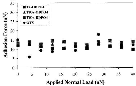
Fig. 7. Adhesion force of specimens with the applied normal load.
