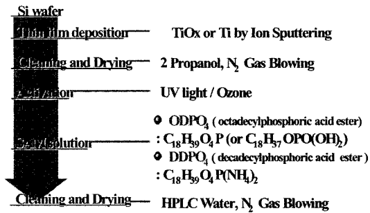
Fig. 3. ODPO 4 and DDPO 4 SAM coating process.
