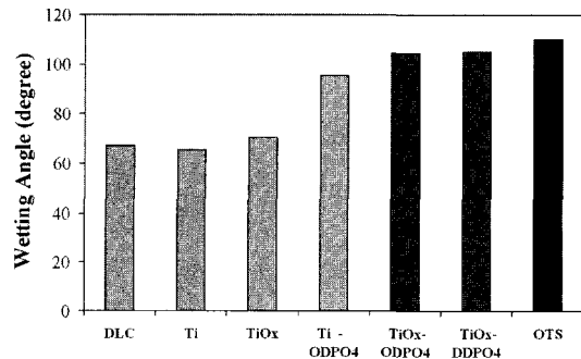
Fig. 5. Wetting angles of the specimens.
