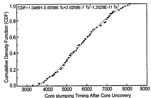
Fig. 1. Core Slumping Timing Produced from MAAP 4 Calculations with 100LHS Samples
