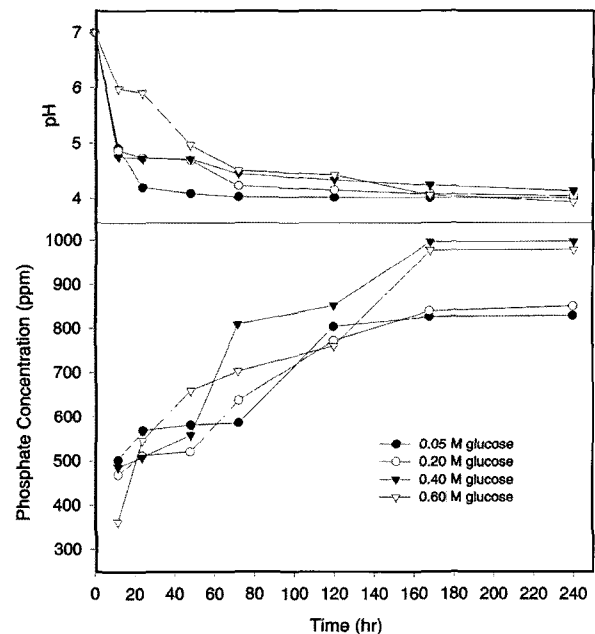
Fig. 4. Changes in pH and phosphate concentration by P. agglomerans over 10 days incubation in broth medium containing 0.4% hydroxyapatite at 30°C in aerated condition.
