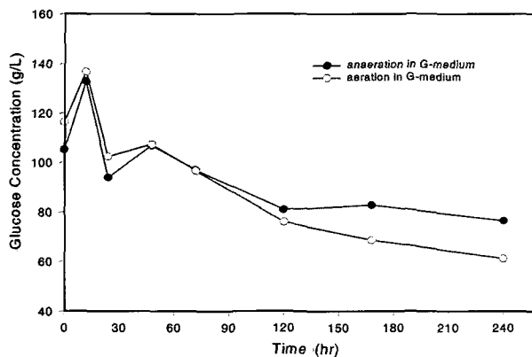
Fig. 6. Changes in glucose concentration by P. agglomerans over 10 days incubation in broth G medium containing 0.8% hydroxyapatite at 30°C.
