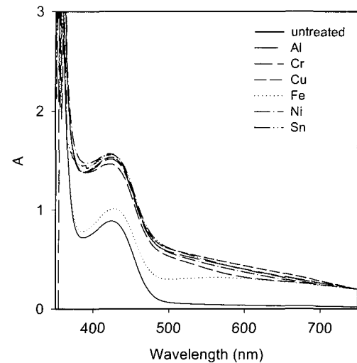
Fig. 11. UV/Vis spectra of extracts containing 5 mg/10ml metal mordants.
