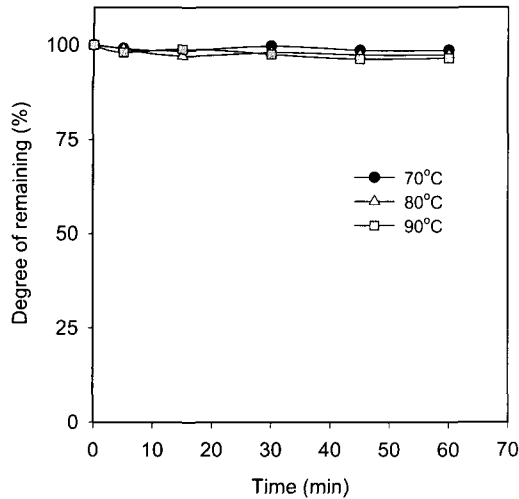
Fig. 9. Relationship between degree of remaining for dye and leaving time at 70, 80, 90 °C. ( \lambda_{max}=428nm )
