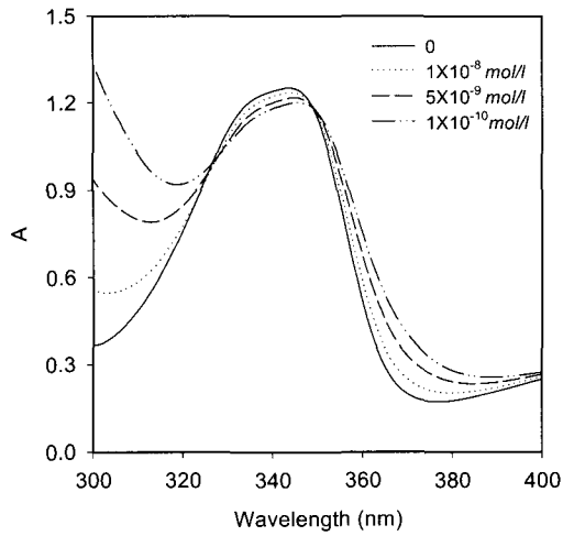
Fig. 12. UV/Vis spectra of 2.5 \times 10^{-4} \text{ mol/l} berberine aqueous solution containing various amounts of tannic acid.
