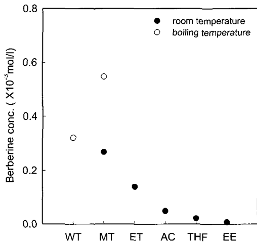
Fig. 2. Berberine concentrations in amur cork tree extracts with water and various organic solvents(WT : water, MT : methanol, ET : ethanol, AC : acetone, THF : tetrahydrofuran, EE : ethyl ether).
