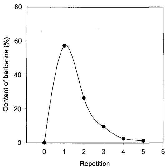
Fig. 4. Relationship between repetition of extraction by methanol and content of berberine in extracts.
