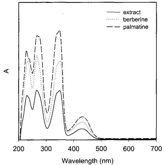
Fig. 8. UV/Vis spectra of berberine, palmatine and extract.
