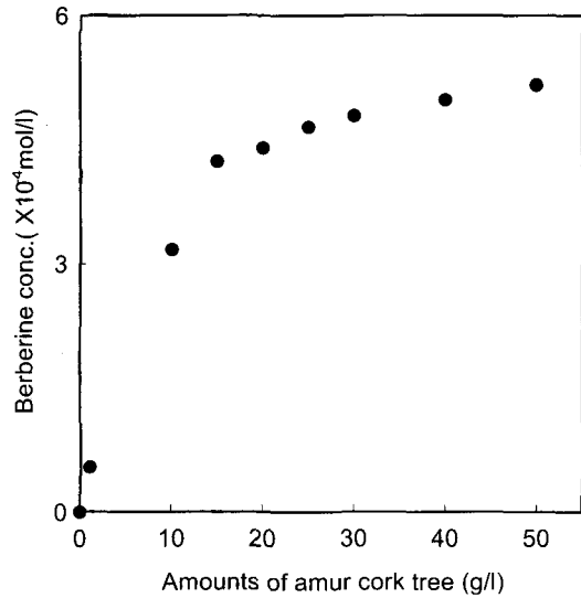
Fig. 3. Relationship between amounts of amur cork tree and berberine concentrations in extracts.
