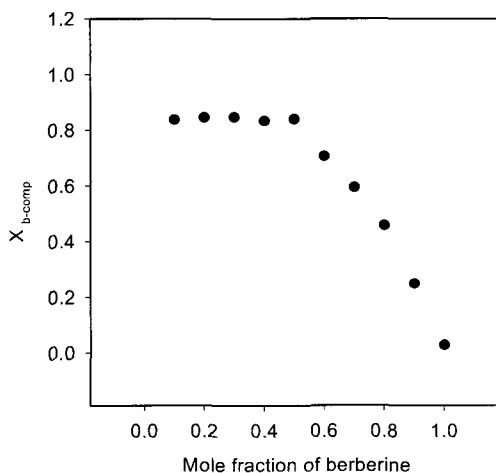
Fig. 13. Effect of mole fraction of berberine on complex formation.
