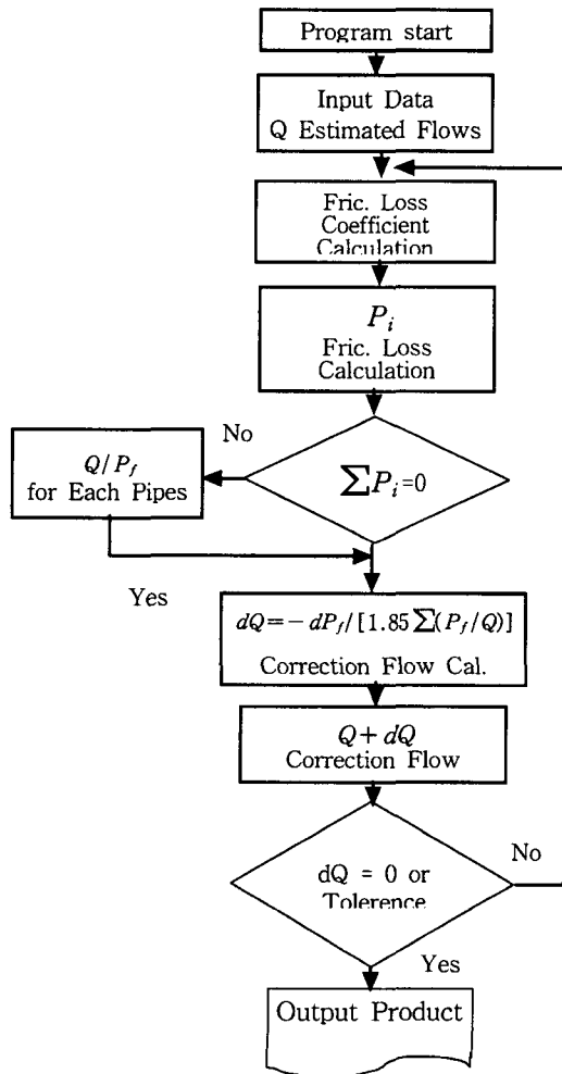
Fig. 2. The algorithm of the program.
