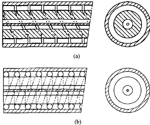
Fig. 2 Shape of new composite reinforced optical fiber jumper cord (OJC). (a) band type composite spring reinforced OJC [B-type], and (b) yarn type composite spring reinforced OJC [Y-type, S-type].
