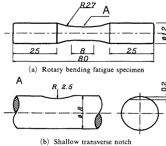
Fig. 1 Configuration of specimen (unit : mm)
