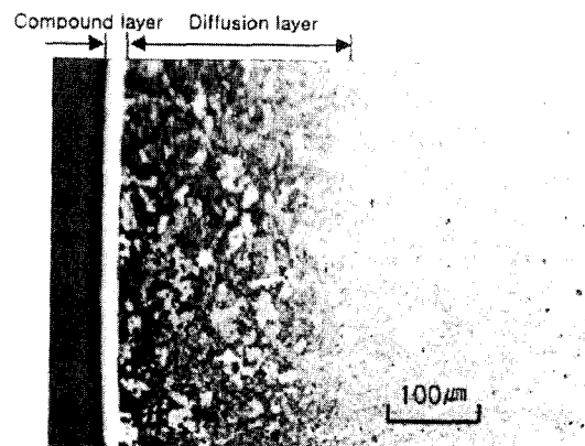
Fig. 3 Microstructure of nitrided layer formed by the single stage heating cycle for 6 hr at 570°C
