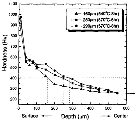
Fig. 4 Micro-Vickers hardness profiles and nitrided depth with different nitriding process
