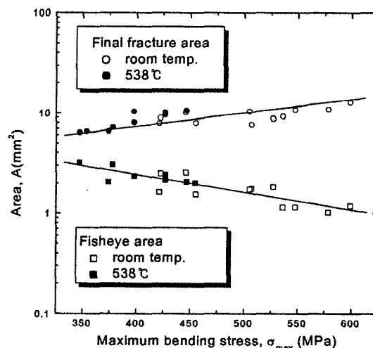
Fig. 7 Behaviors of the fish-eye and the final fractured area with the maximum applied bending stress
