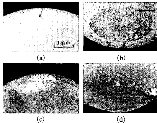
Fig. 6 Fractographs of fish-eye and final fracture pattern for 250 \mu m nitrided specimen: (a) and (b) at \sigma_a=407 MPa, N_f=1.05 \times 10^7 , RT; (c) and (d) at \sigma_a=454 MPa, N_f=1.04 \times 10^5 , 538 ^{\circ} C
