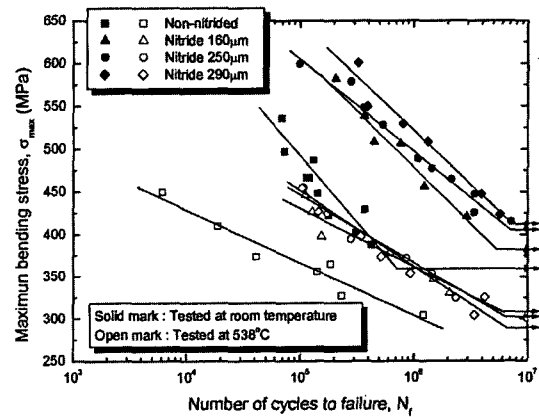
Fig. 5 Relationship between maximum bending stress, \sigma_{\text{max}} and number of cycles to failure, N_f at room temperature and 538 °C
