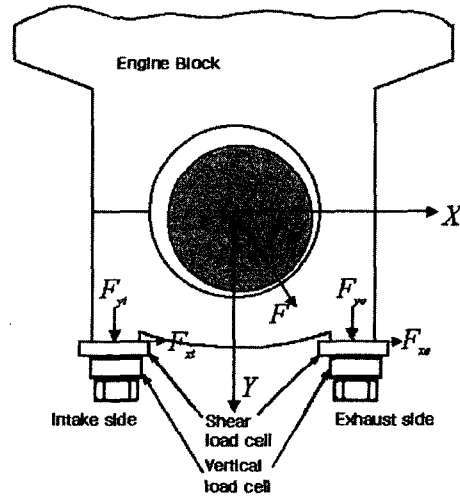
Fig. 3 Schematic diagram of load cell mounting
