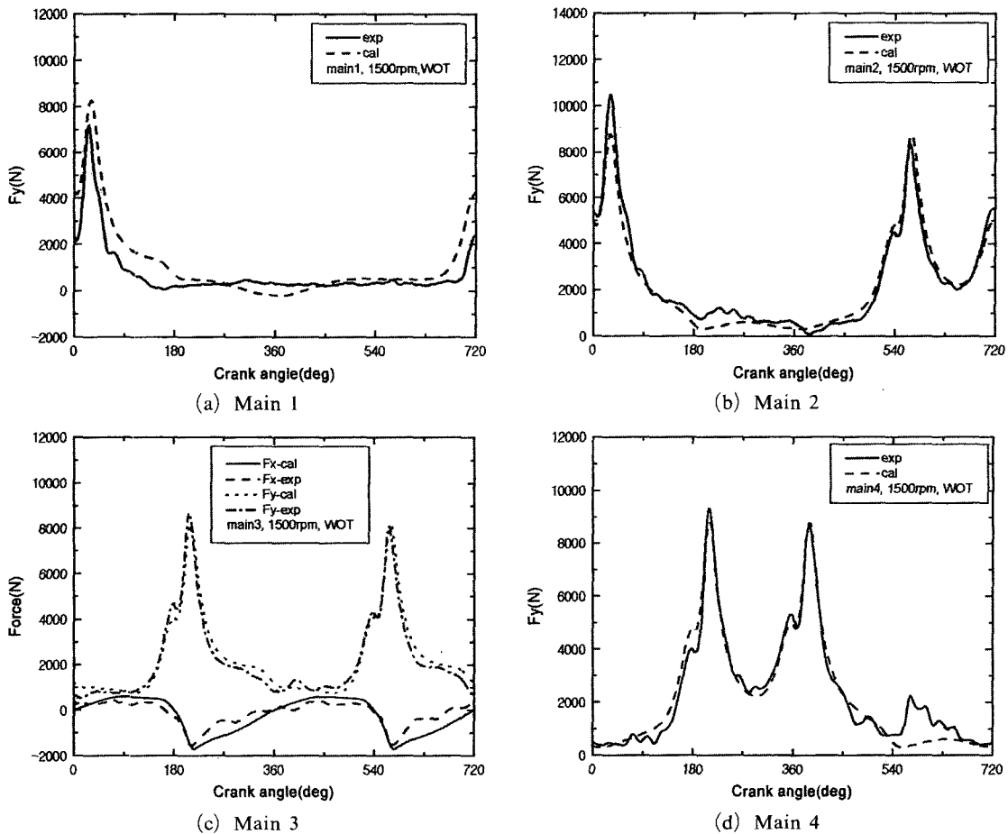
Fig. 5 The experimental and calculated bearing load in each main bearing
