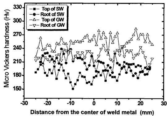
Fig. 3 Hardness distribution of the weld metals
