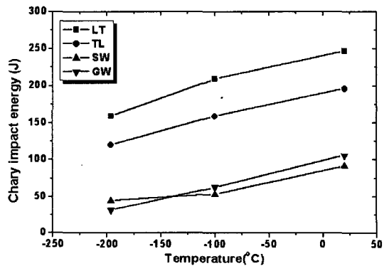
Fig. 5 Charpy impact energy of the base metal and weld metals
