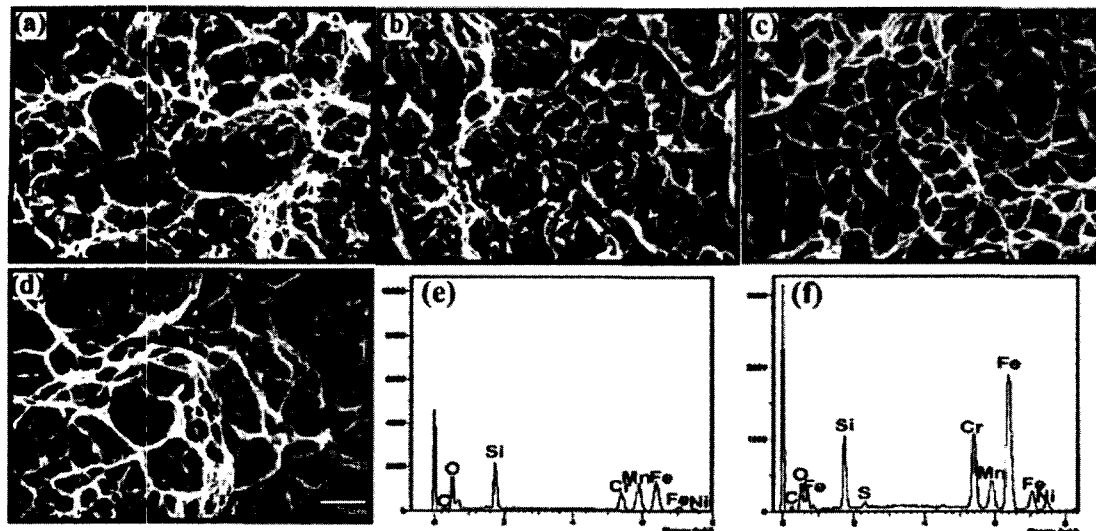
Fig. 6 SEM photographs and EDS of the base and weld metal on the Charpy impact specimens at -196^{\circ}\text{C} : (a) LT of BM, (b) TL of BM, (c) SW, (d) GW, (e) EDS of Fig. 6(c), (f) EDS of Fig. 6(d)
