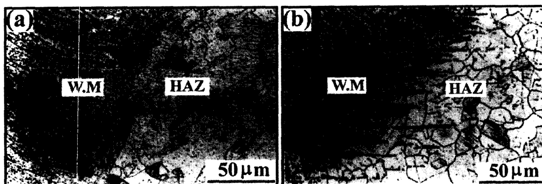
(a) Weld metal/HAZ of seam welds
