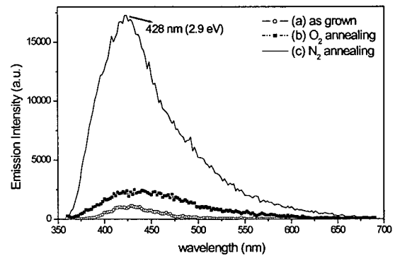
Fig. 1 Room temperature PL spectra from three samples of as deposited, after annealing at 760°C for 10 min. in O 2 and after annealing at 760°C for 10 min. in N 2 .
