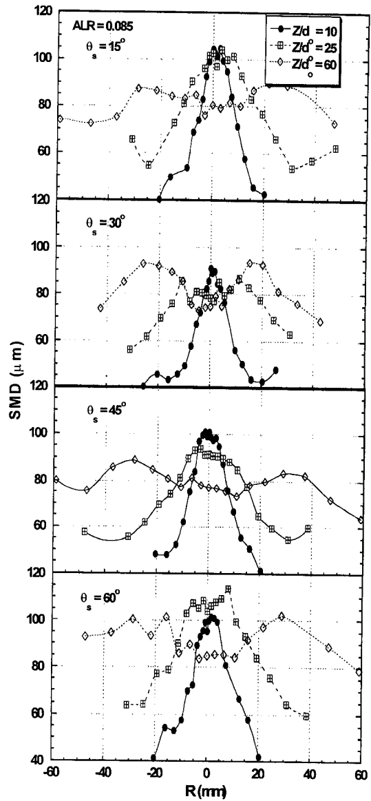
Fig. 8 Distributions of sauter mean diameter different swirl angles measured at three axial downstream locations
