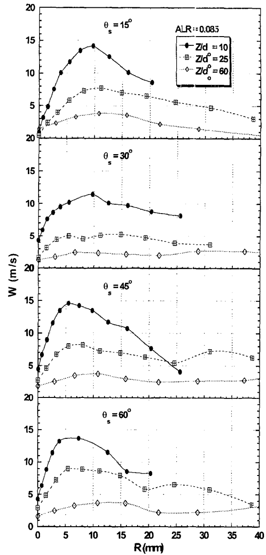
Fig. 6 Distributions of tangential mean velocity for different swirl angles measured at three axial downstream locations
