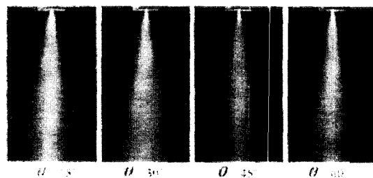
Fig. 3(b) Photographic visualization for the higher ALR
