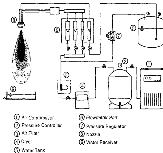
Fig. 2 Schematic set up for the experimental apparatus
