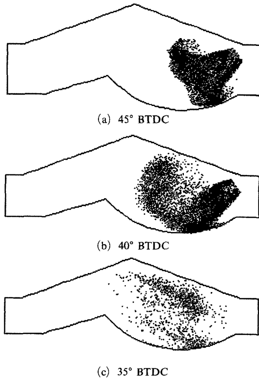
Fig. 9 Calculated results of spray shapes for the type 2
