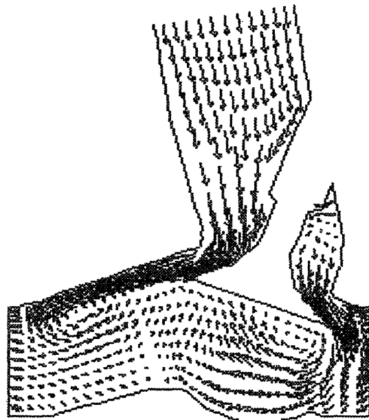
Fig. 4 Velocity vectors for the type 2
