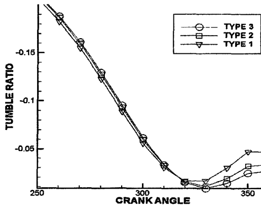
Fig. 6 Tumble ratios for three types
