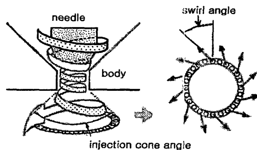
Fig. 1 Schematic of the Nozzle Outlet
