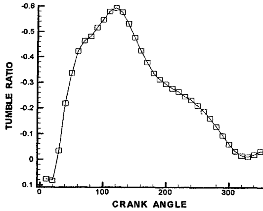
Fig. 5 Tumble ratio for the type 2
