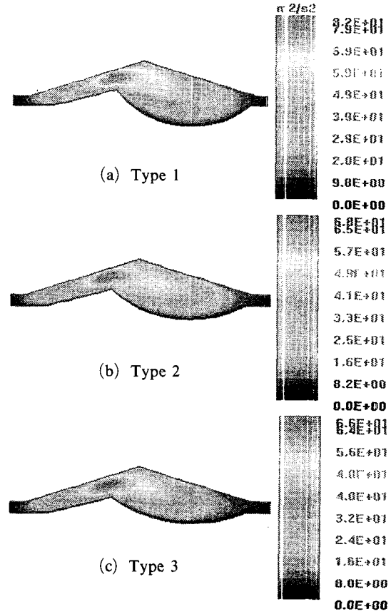
Fig. 7 The distributions of turbulent kinetic energy (at BTDC 10°)
