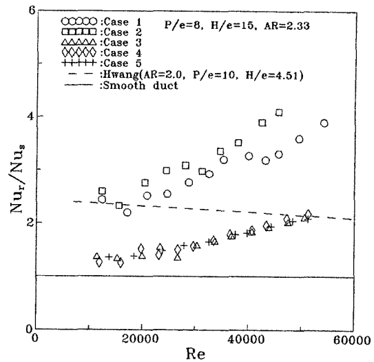
Fig. 5 Normalized Nusselt number
