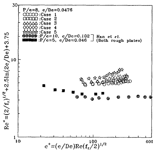
Fig. 6 Roughness function
