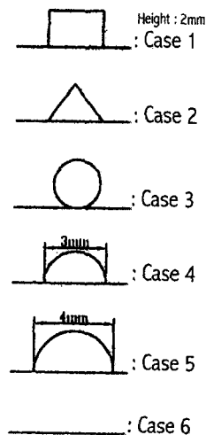
Fig. 2 Rib shape
