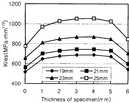
Fig. 13 SIF in the thickness direction according to crack length
