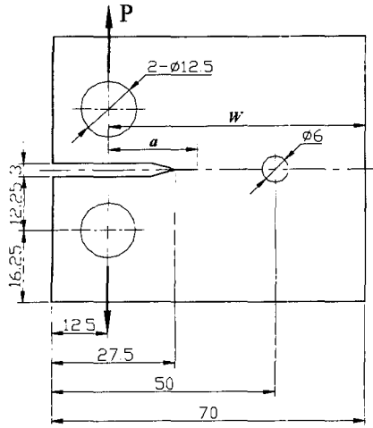
Fig. 4 Geometry of CT specimen
