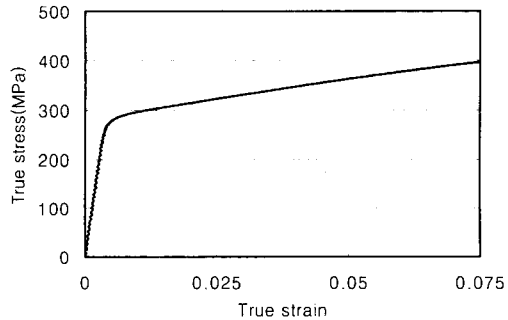
Fig. 3 True stress-strain relation of Al6061-T6
