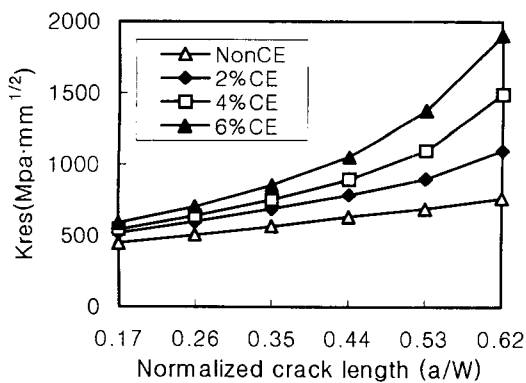
Fig. 14 SIF according to cold expansion ratio
