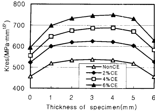
Fig. 12 SIF of thickness direction according to cold expansion ratio
