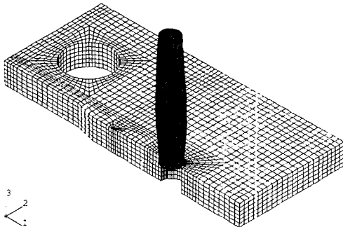
Fig. 5 Half modeling
