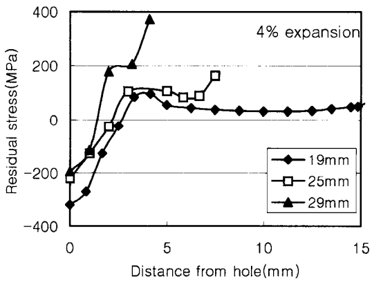
Fig. 10 Residual stress by cold expansion for different crack lengths
