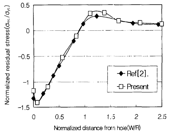
Fig. 8 Residual stress distribution at mid thickness in the case of 4% cold expansion
