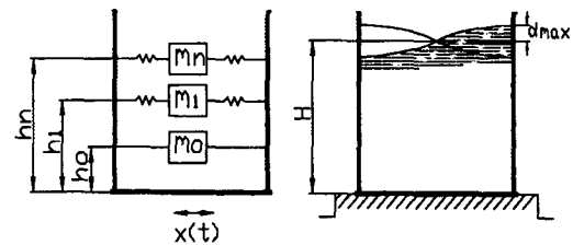
Fig. 2 Equivalent model and fluid motion
