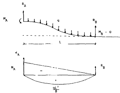
Fig. 7 Equilibrium diagram for lifted bottom plate
