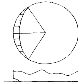
Fig. 6 Fluid area contributing to resistance
