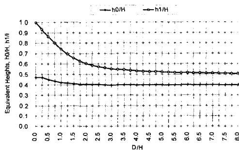
Fig. 5 Equivalent heights
