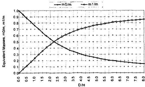
Fig. 4 Equivalent masses
