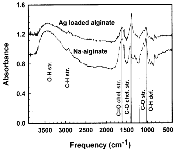
Figure 1. Fourier transformed infrared spectra from Na-alginate or Ag loaded alginate. 50 mg KBr disks for FT-IR contained 10% of finely powdered materials. str.=stretching, chel. str.=chelate stretching, def.=deformation.
