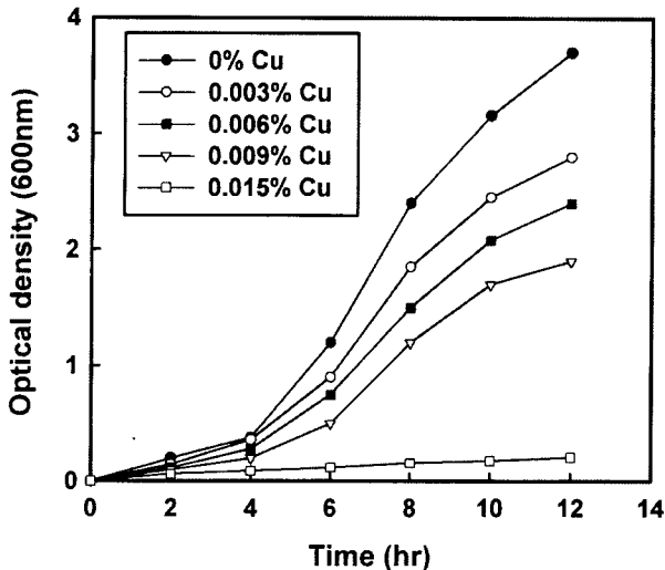
Figure 6. Antibacterial effect of Cu-alginate for S. aureus at pH 7.
