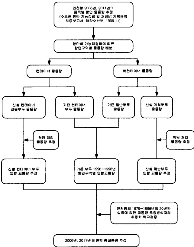
Fig. 2 Flow Chart to estimate Traffic Volumes in Incheon Port(Year: 2006, 2011)
