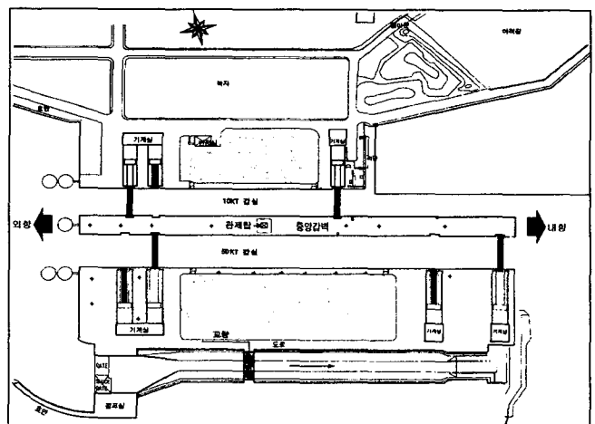
Fig. 1 Layout of Lock Gates in Incheon Port
