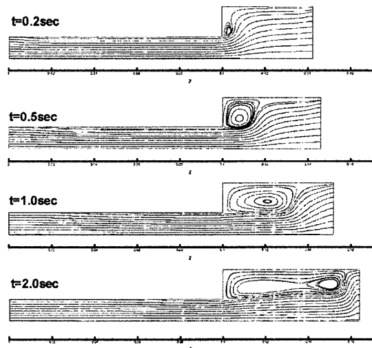
Fig. 18 Streamlines at t=0.2s, 0.5s, 1.0s and 2.0s
