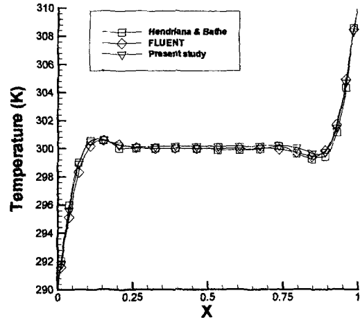
Fig. 8 The temperature values along y=0.5
