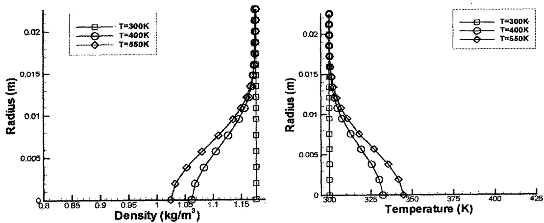
Fig. 22 Density and temperature profiles at z=0.1319m
