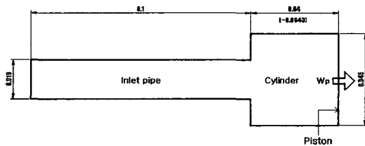
Fig. 11 Piston-cylinder configuration
