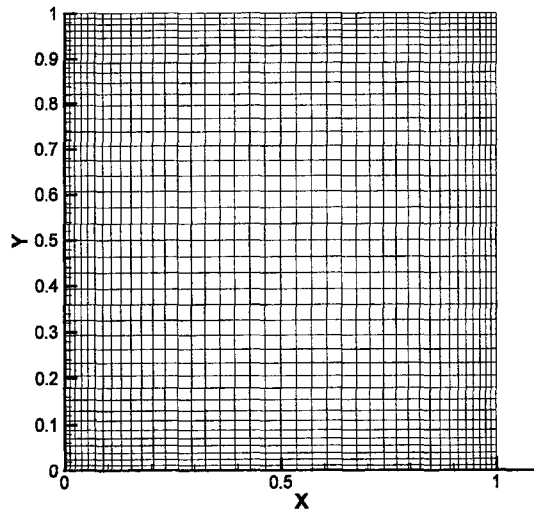
Fig. 5 Nonuniform 41 \times 41 grid system for natural convection problem
