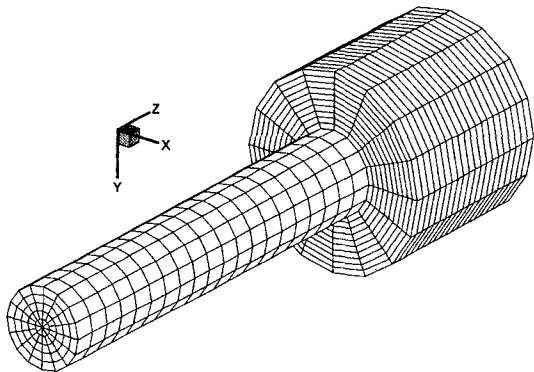
Fig. 12 The mesh used for piston-driven intake flow
