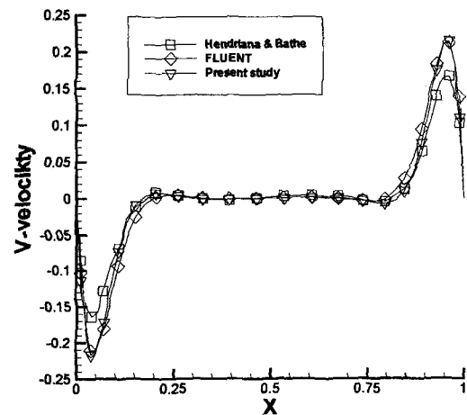
Fig. 9 The y-direction velocity values along y=0.5
