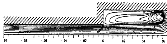
Fig. 14 Streamlines obtained by 2-D FVM
