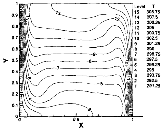
Fig. 7 The temperature distribution for natural convection problem
