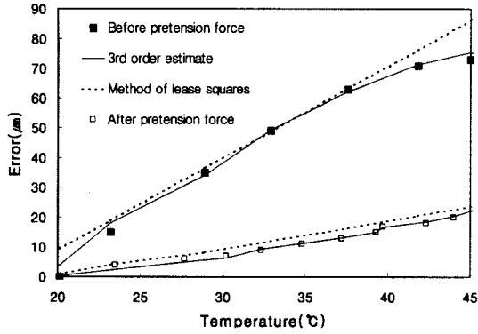
Fig. 6 Variation in temperature with error for experiment in the DT type
