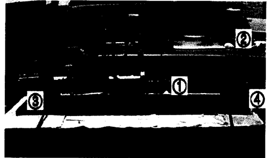
① Fix bearing ② Ball screw ③ Gap sensor ④ Support bearing
