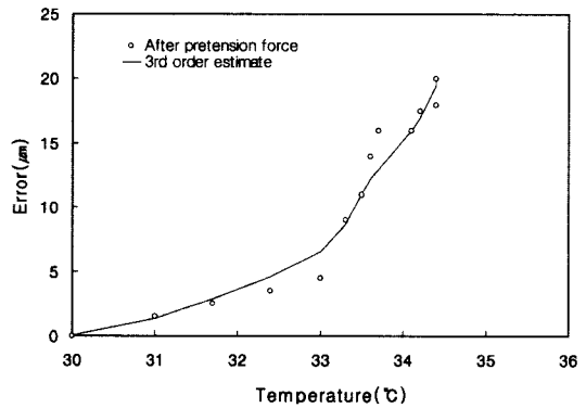
Fig. 9 Relation between temperature and error for experiment in the D type
