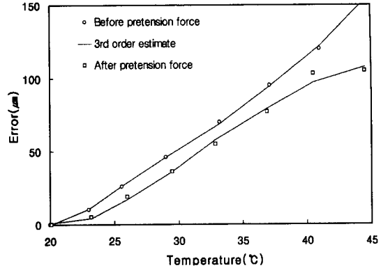
Fig. 5 Variation in temperature with error for experiment in the D type
