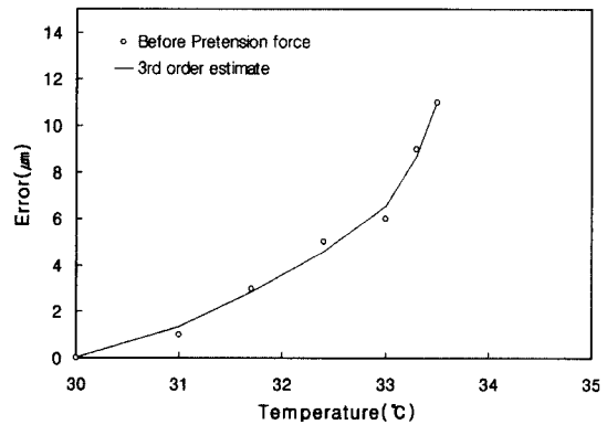
Fig. 10 Relation between temperature and error for experiment in the DF type
