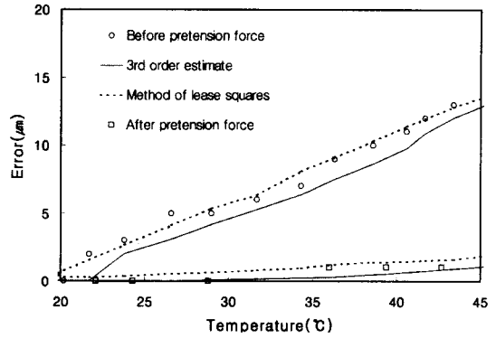
Fig. 7 Variation in temperature with error for experiment in the DBD type
