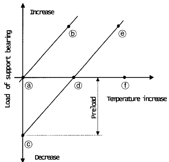
Fig. 2 Relation between load of support bearing and temperature increase
