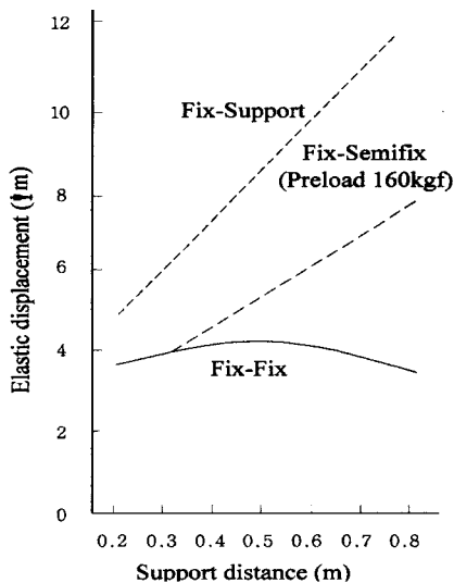
Fig. 1 Relation between elastic displacement and support distance
