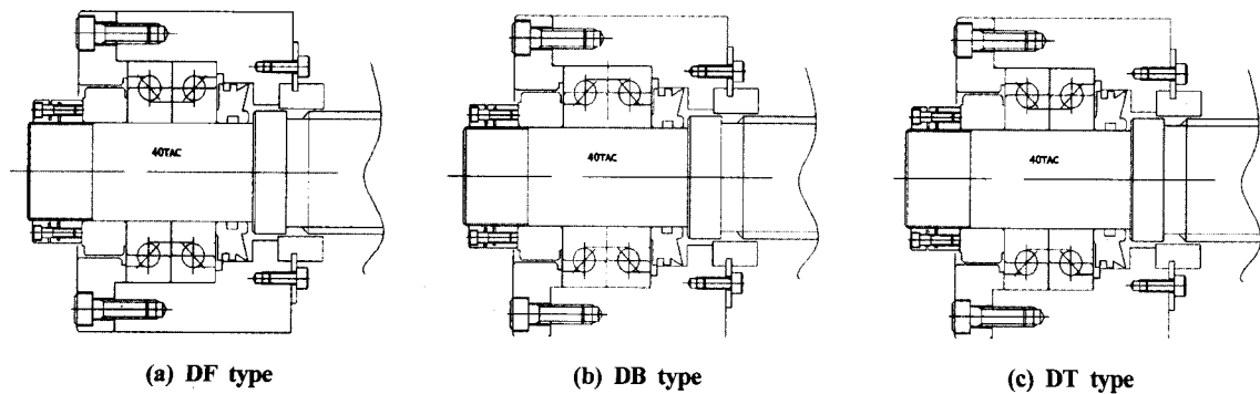
Fig. 3 Supporting fix-semi fix for DF, DB, DT type
