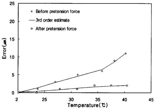
Fig. 8 Variation in temperature with error for experiment in the DBT type
