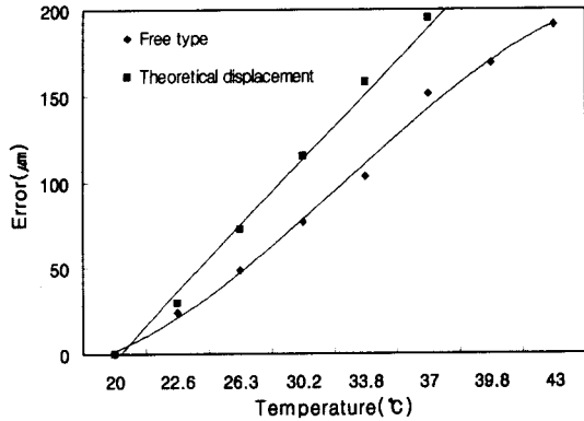
Fig. 4 Variation in temperature with error for experiment in the free type
