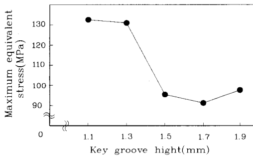
Fig. 10 Stress value according to change of key groove height
