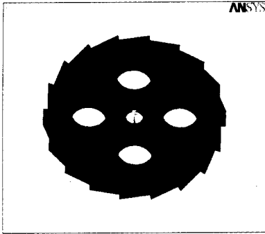
Fig. 5 Finite element model of ratchet wheel
