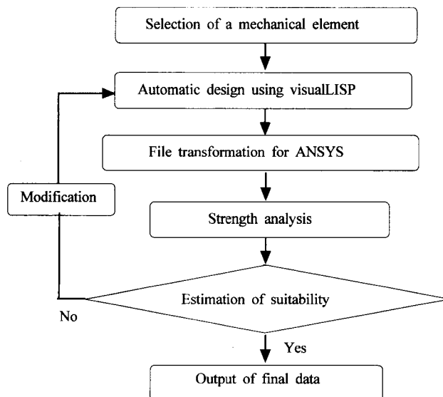
Fig. 4 Method of Inspection for optimum shape design using automatic design program and FEA
