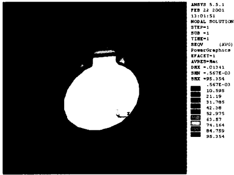
Fig. 9 Distributed equivalent stress when key width is 4 mm & key height is 1.5 mm
