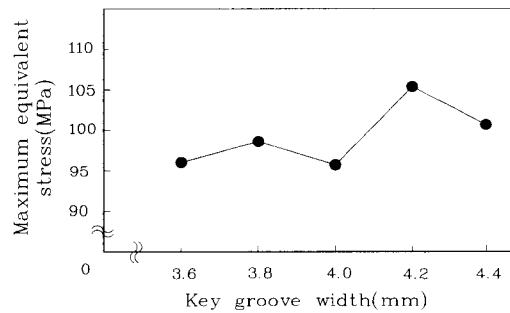
Fig. 11 Stress value according to change of key groove width
