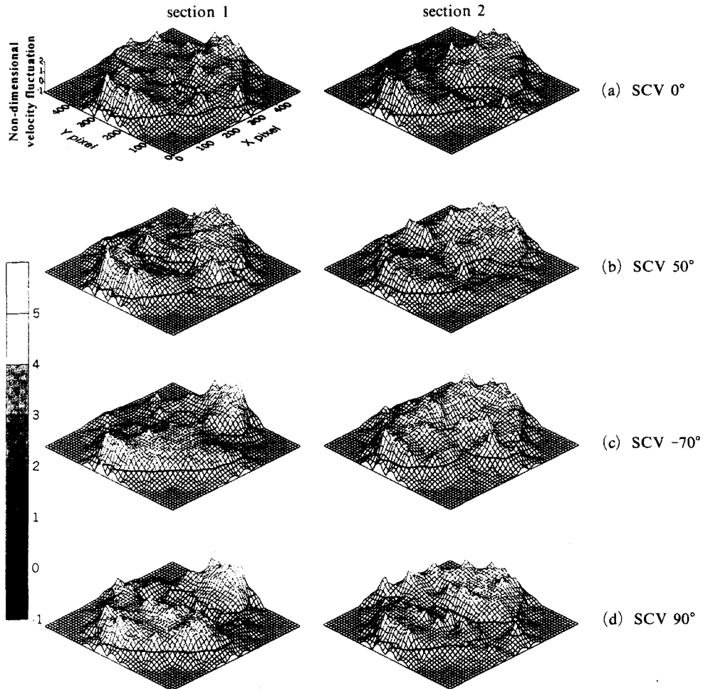
Fig. 13 Distribution of non-dimensional velocity fluctuation
