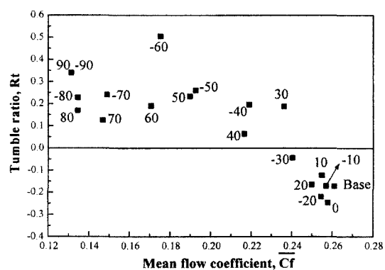
Fig. 8 Correlation between mean flow coefficient and tumble ratio
