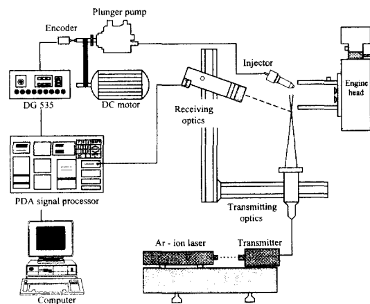
Fig. 3 Schematic diagram of PDA experiment
