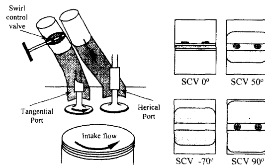
Fig. 1 Geometry and definition of SCV opening angle
