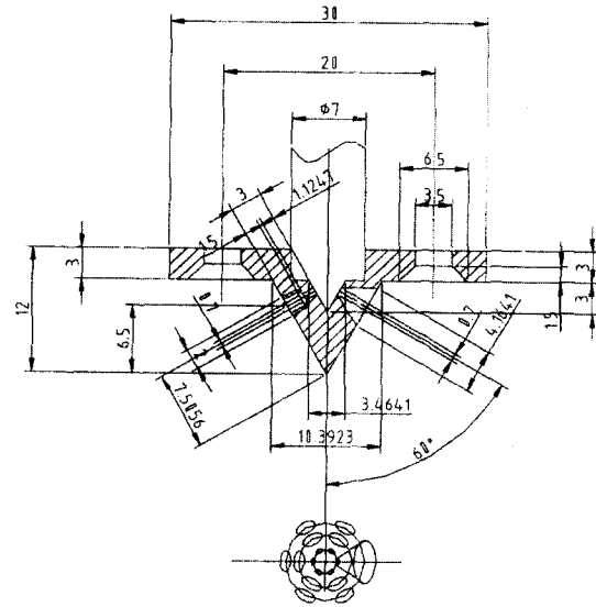
Fig. 5 Drawing the VCO nozzle cap
