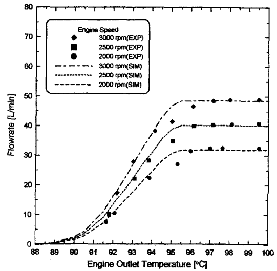
Fig. 7 Variation of coolant flowrate with engine outlet coolant temperature
