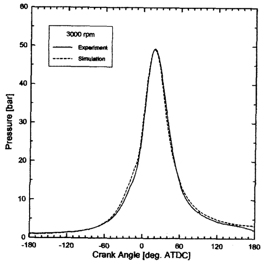
Fig. 5 Cylinder pressure diagram at 3000rpm and W.O.T
