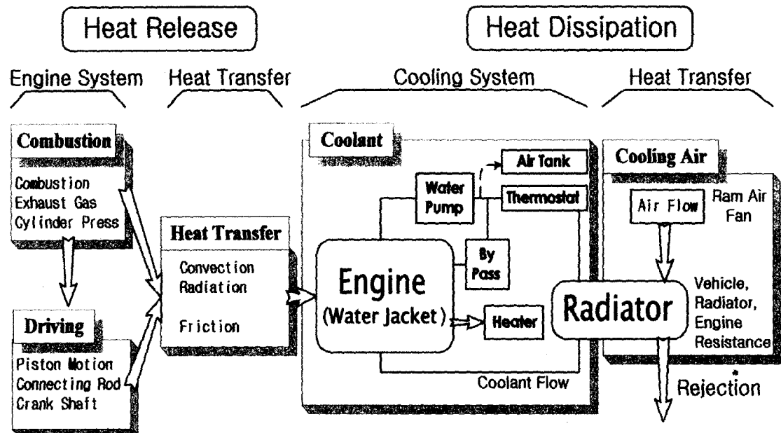
Fig. 1 Automotive engine cooling systems
