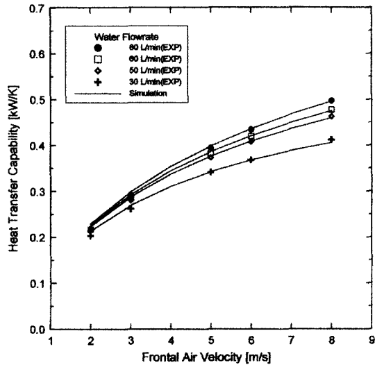
Fig. 8 Radiator Heat Dissipation Characteristics
