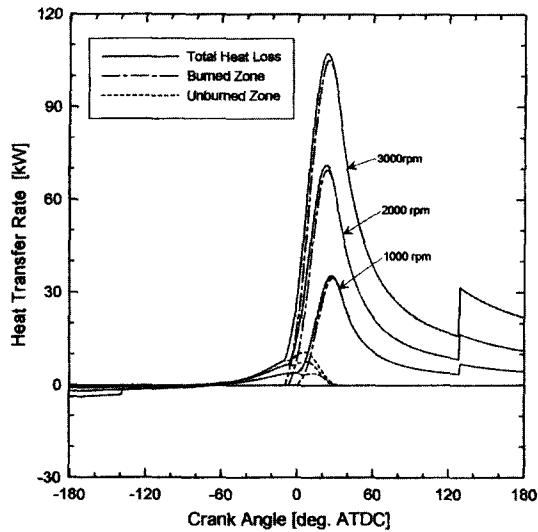
Fig. 6 Overall in-cylinder heat transfer rate
