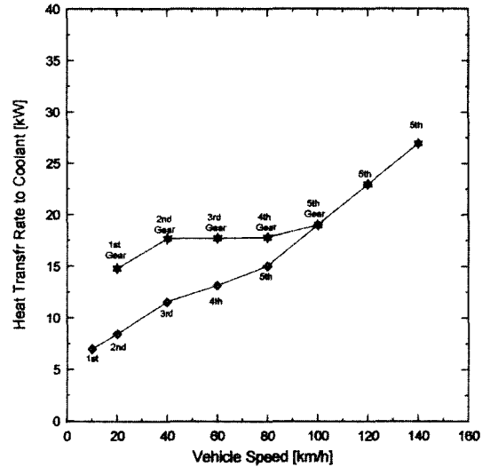
Fig. 9 Variation of heat transfer rate to coolant with vehicle speed
