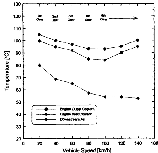
Fig. 10 Variation of coolant temperature with vehicle speed (CASE 1)
