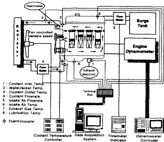
Fig. 4 Schematic diagram of cooling system experimental apparatus
