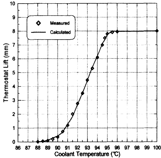
Fig. 2 Thermostat characteristics
