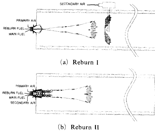
Fig. 5 Sketch of the reburn-mode I and II
