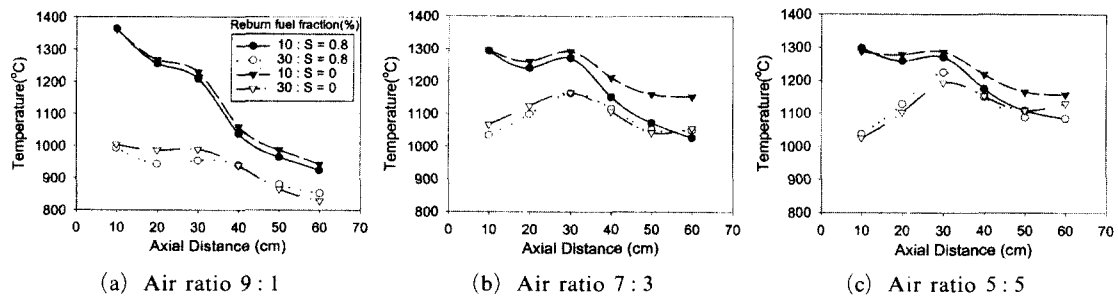
Fig. 13 Temperature distribution on axial direction in reburn fuel Fraction
