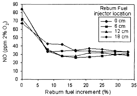
Fig. 8 NOx emission level versus reburn-fuel increment
