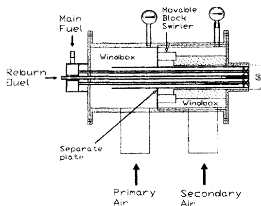
Fig. 4 Detailed configuration of burner
