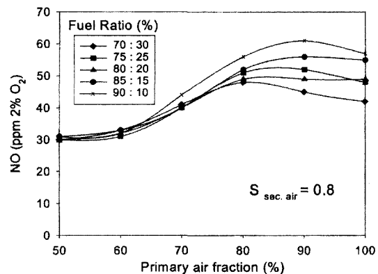
Fig. 11 Effect of primary-air fraction on NO emission
