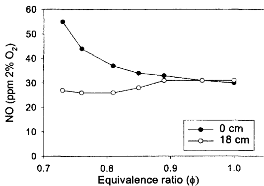
Fig. 9 Effect of primary-zone stoichiometry on NOx emission
