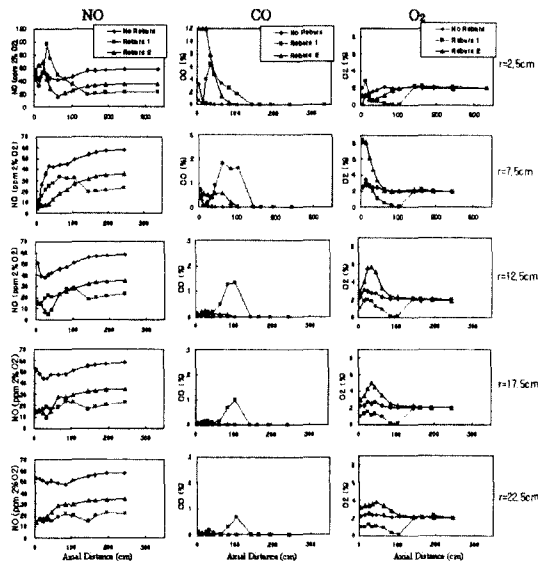
Fig. 15 Emission profile comparison in furnace
