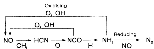
Fig. 2 Reaction pathways in the reburning process
