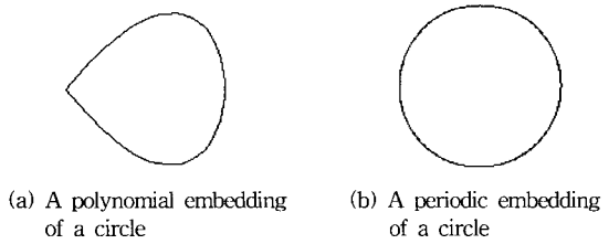
Fig. 2. Periodizing transformation
