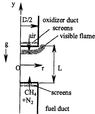
Fig. 1 A schematic diagram of the counterflow ducts and notations
