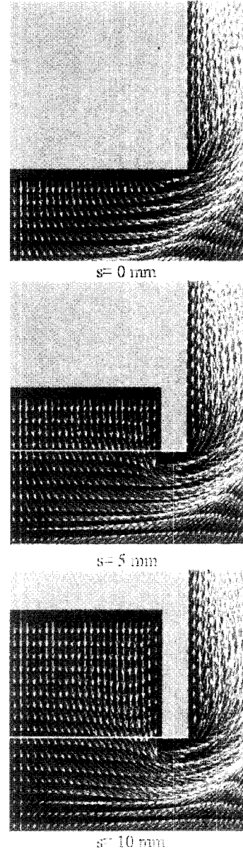
Fig. 7 Velocity vectors around the oxidizer duct exit at a_g=20\text{ s}^{-1} for different values of s
