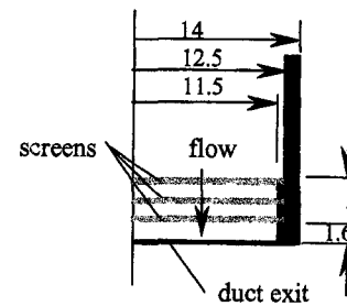
Fig. 2 Dimensions of the screens and the duct near the exit in mm, nonscale
