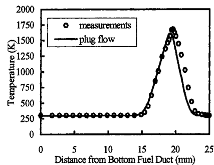
Fig. 11 Comparison of flames at a_g=20 s -1 ( s=2 mm)
