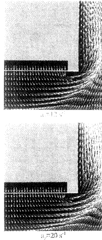
Fig. 9 Velocity vectors around the oxidizer duct exit ( s=2 \text{ mm} )
