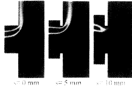
Fig. 3 High temperature reaction zone for steady flames of a_g=12 s^{-1} for different values of s
