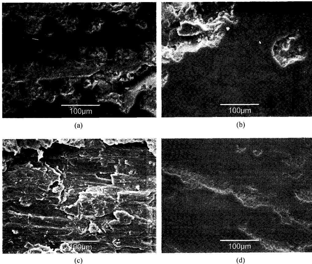
Fig. 9. SEM images of the worn surface of the discs; (a) CrO and (b) CrMO20 from self-mated tests, (c) CrO and (d) CrMO5 from Cr plated disc/plasma spray-coated plate tests.
