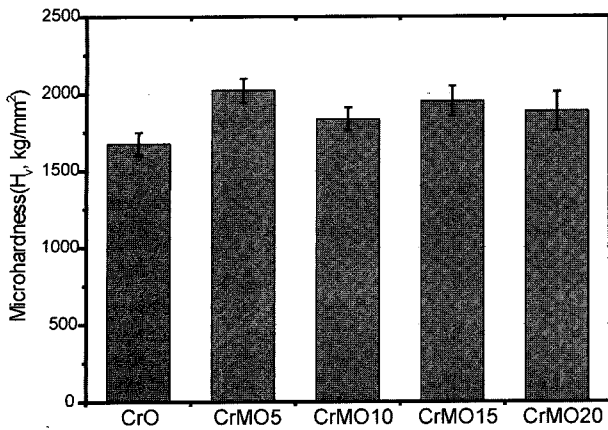
Fig. 4. Vickers microhardness values of plasma spray-coated discs.
