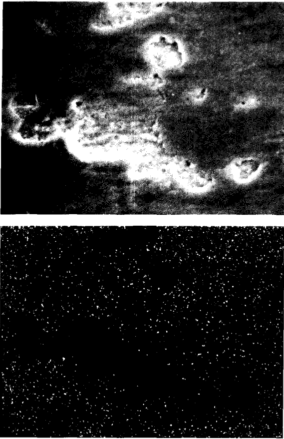
Fig. 10. SEM image and the dot map of the Mo distribution at the worn surface of Cr-plated disc.
