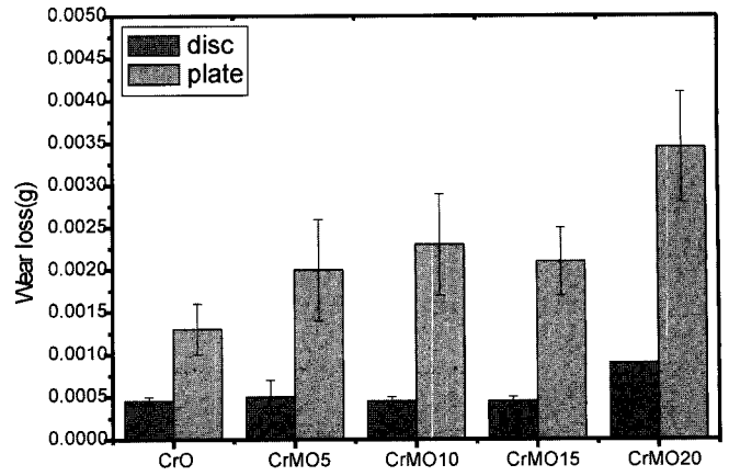
Fig. 6. Wear loss of specimens for self-mated Cr 2 O 3 -MoO 3 coatings.
