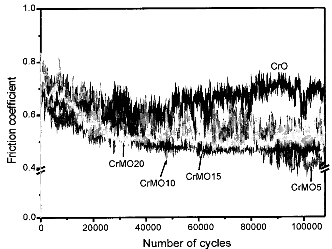
Fig. 7. Coefficient of friction vs. number of cycles for Cr-plated disc/plasma spray-coated plate.
