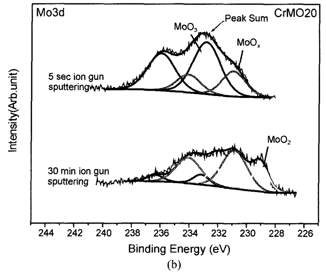
Fig. 12. X-ray photoelectron spectra of the worn surface.; (a) Cr2p and (b) Mo3d of CrMO20.
