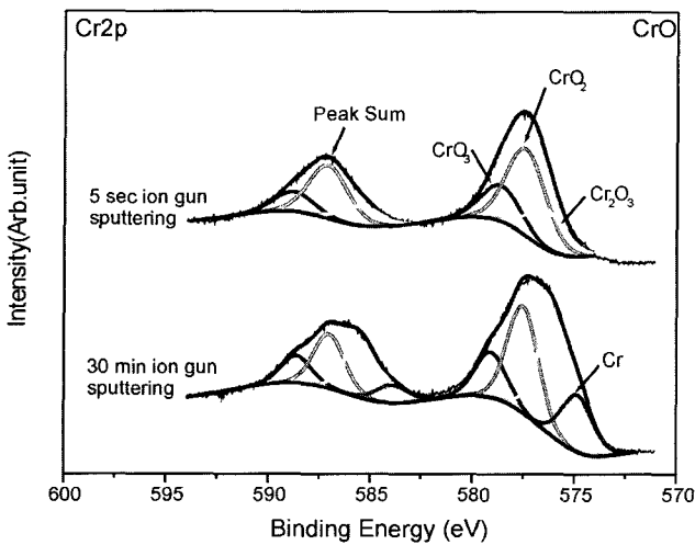
Fig. 11. Cr2p X-ray photoelectron spectra of the worn surface tested of CrO specimen.
