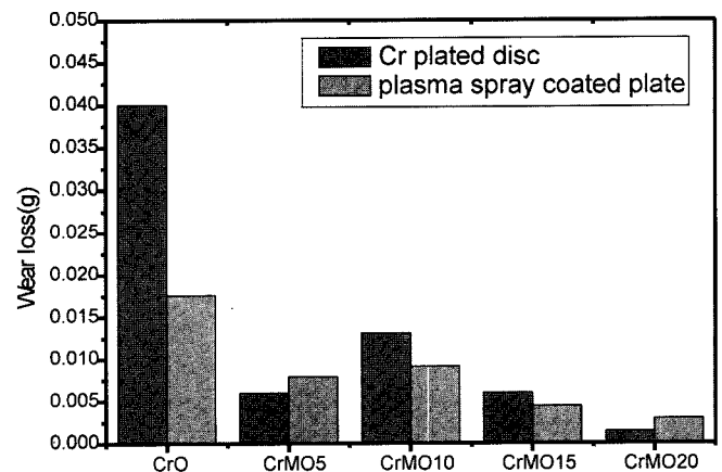
Fig. 8. Wear loss of Cr-plated disc/plasma spray-coated plate.
