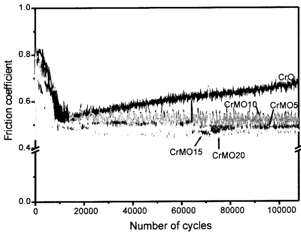
Fig. 5. Coefficient of friction vs. number of cycles for self-mated Cr 2 O 3 -MoO 3 coatings.
