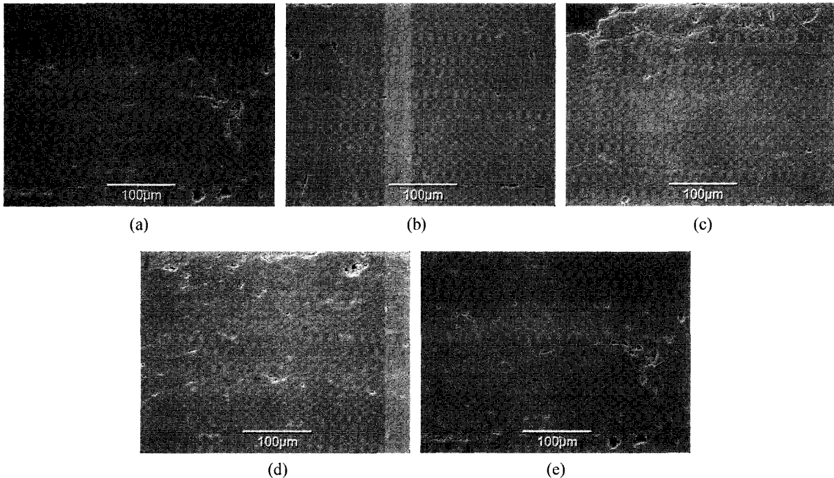
Fig. 2. Cross-sectional SEM images of the Cr 2 O 3 -MoO 3 coated discs; (a) CrO, (b) CrMO5, (c) CrMO10, (d) CrMO15 and (e) CrMO20.
