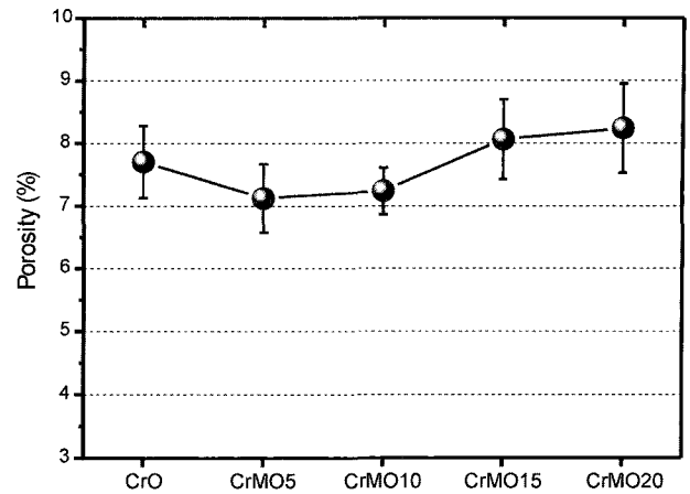
Fig. 3. Porosity values of the plasma splay-coated discs.
