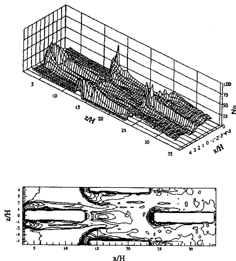
Fig. 6 Distribution of local Nusselt number for fin-flat tube heat exchanger without vortex generators
