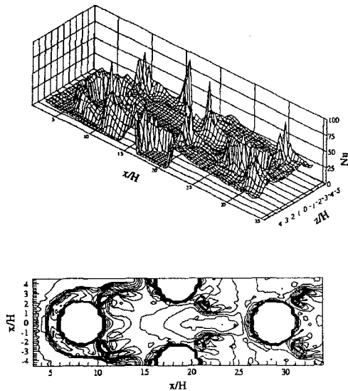
Fig. 3 Distribution of local Nusselt number for fin-circular tube heat exchanger with vortex generators
