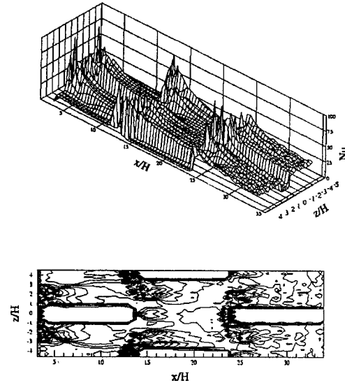
Fig. 7 Distribution of local Nusselt number for fin-flat tube heat exchanger with vortex generators
