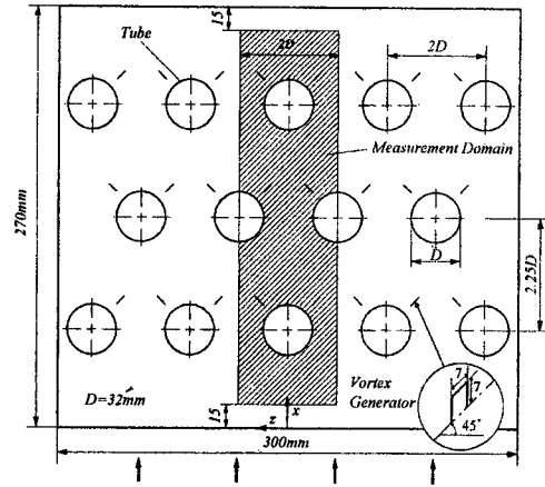
Fig. 1 Schematic of fin-circular tube heat exchanger model
