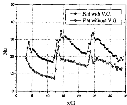
Fig. 8 Comparison of spanwise-averaged heat transfer for fin-flat tube heat exchanger
