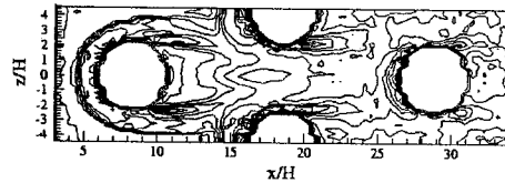
Fig. 2 Distribution of local Nusselt number for fin-circular tube heat exchanger without vortex generators
