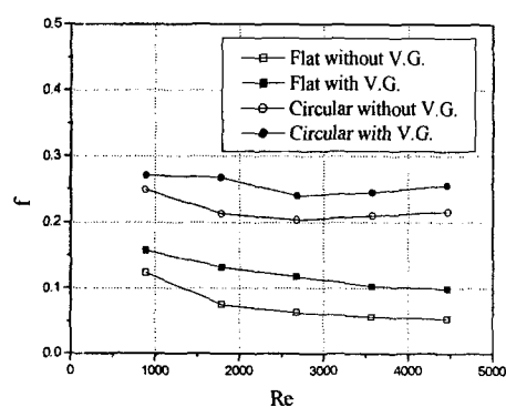
Fig. 9 Comparison of apparent friction factors for four types of heat exchanger
