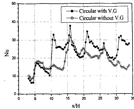
Fig. 4 Comparison of spanwise-averaged heat transfer for fin-circular tube heat exchanger
