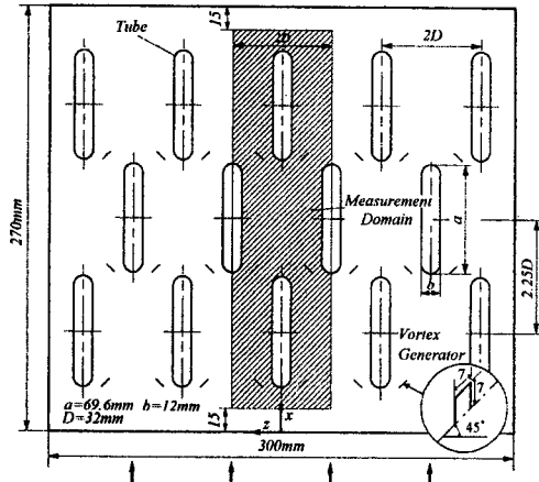
Fig. 5 Schematic of fin-flat tube heat exchanger model
